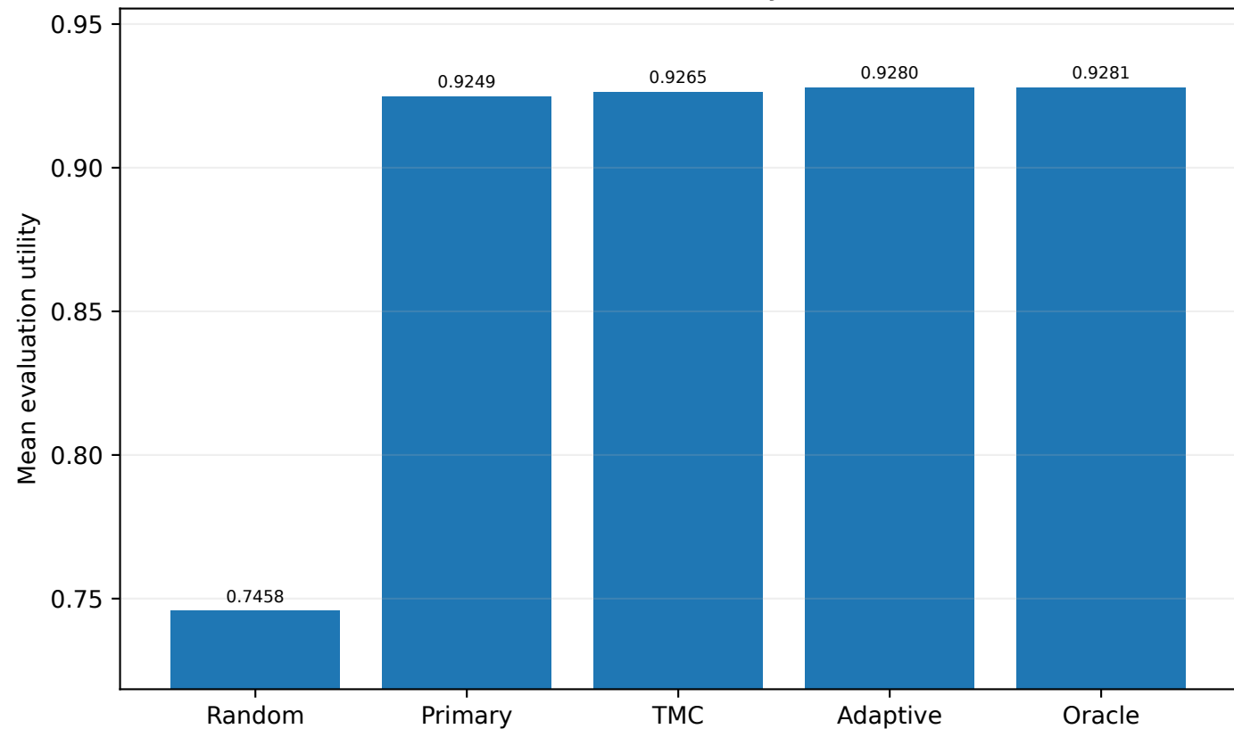
Held-out utility
