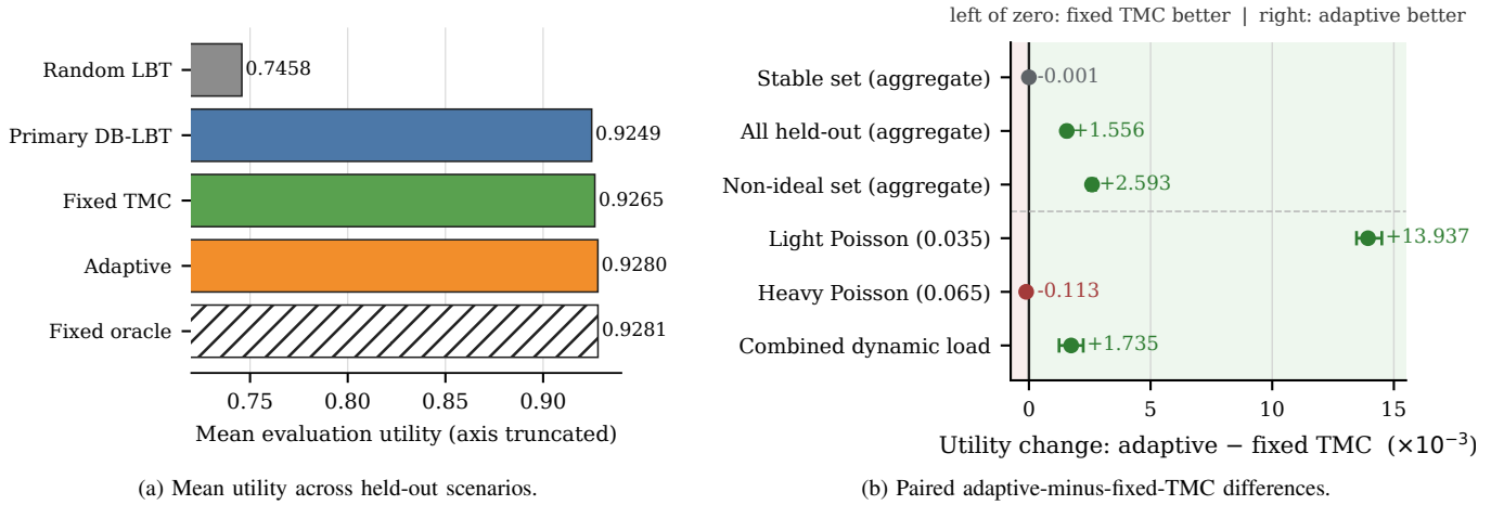
Fig. 2. Held-out event evaluation over ten paired seeds. In (a), the axis is truncated and values are printed beside the bars. In (b), differences are scaled by 10^3 ; bars are 95% paired-bootstrap intervals. Green favors adaptive DB-LBT, red favors fixed TMC, and gray crosses zero.
