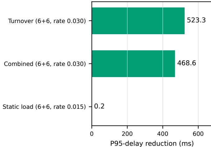
Latency mechanism
