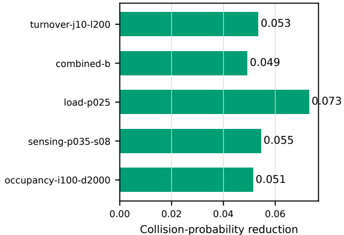
Dominant mechanism
