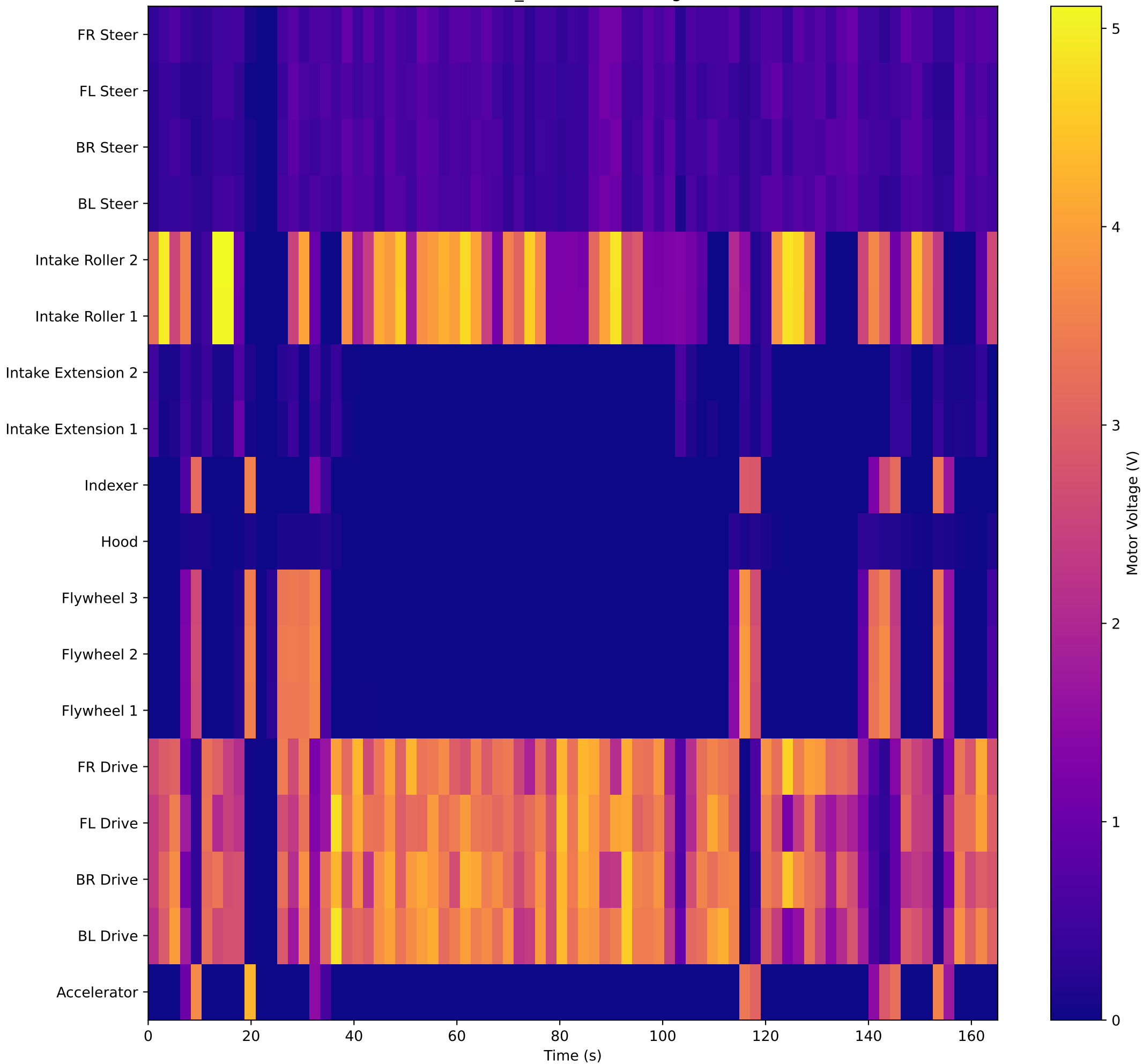
GACMP_E5 — Motor Voltage
