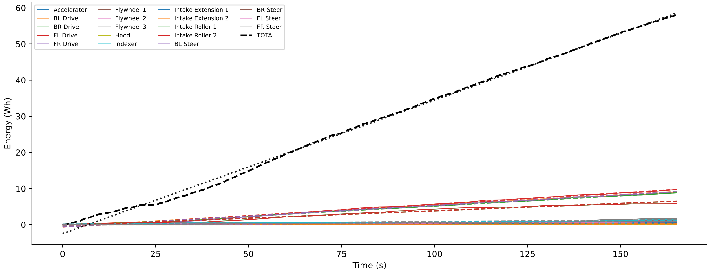
GACMP_E5 — Cumulative Supply Energy
