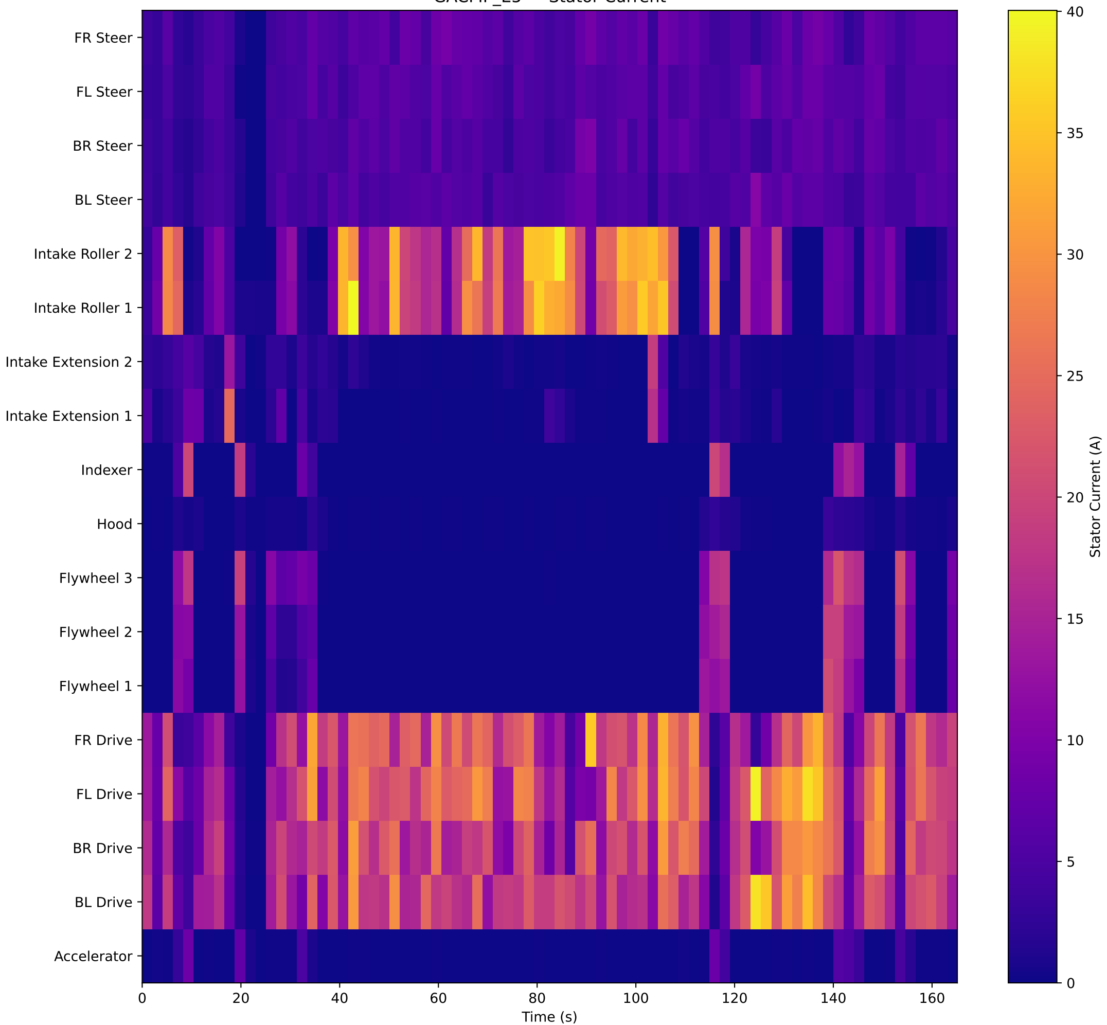
GACMP_E5 — Stator Current
