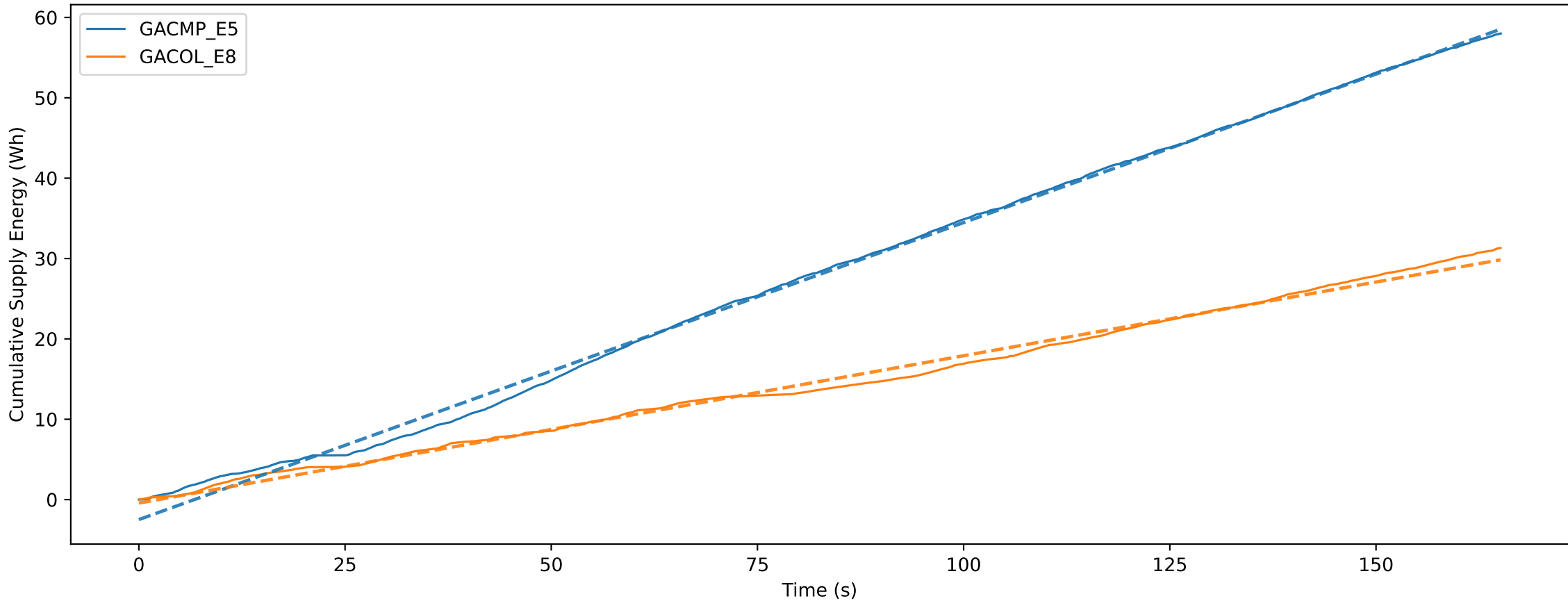
Match Comparison — Cumulative Supply Energy (Robot Total)
