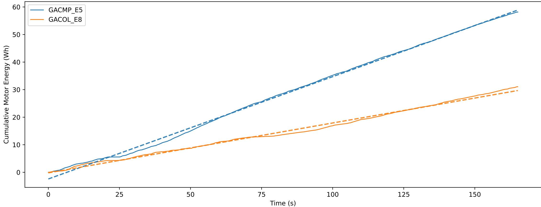
Match Comparison — Cumulative Motor Energy (Robot Total)
