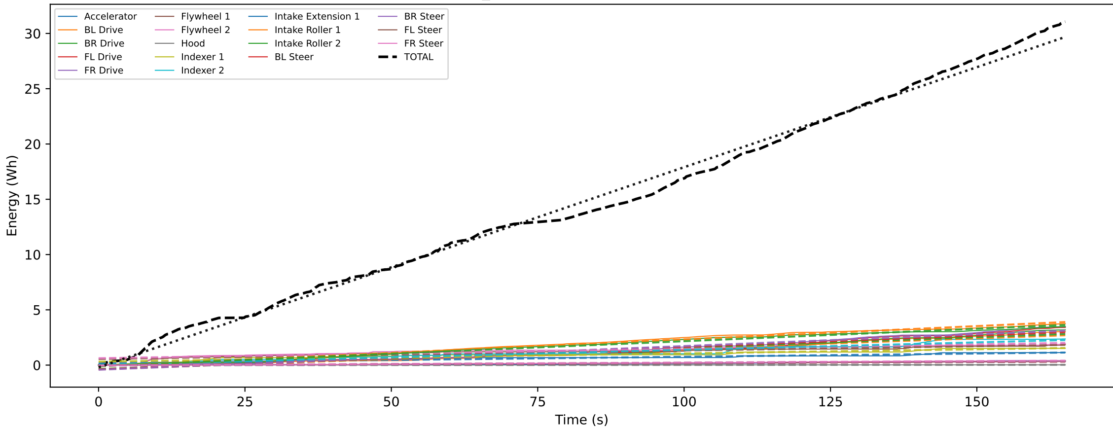
GACOL_E8 — Cumulative Motor Energy
