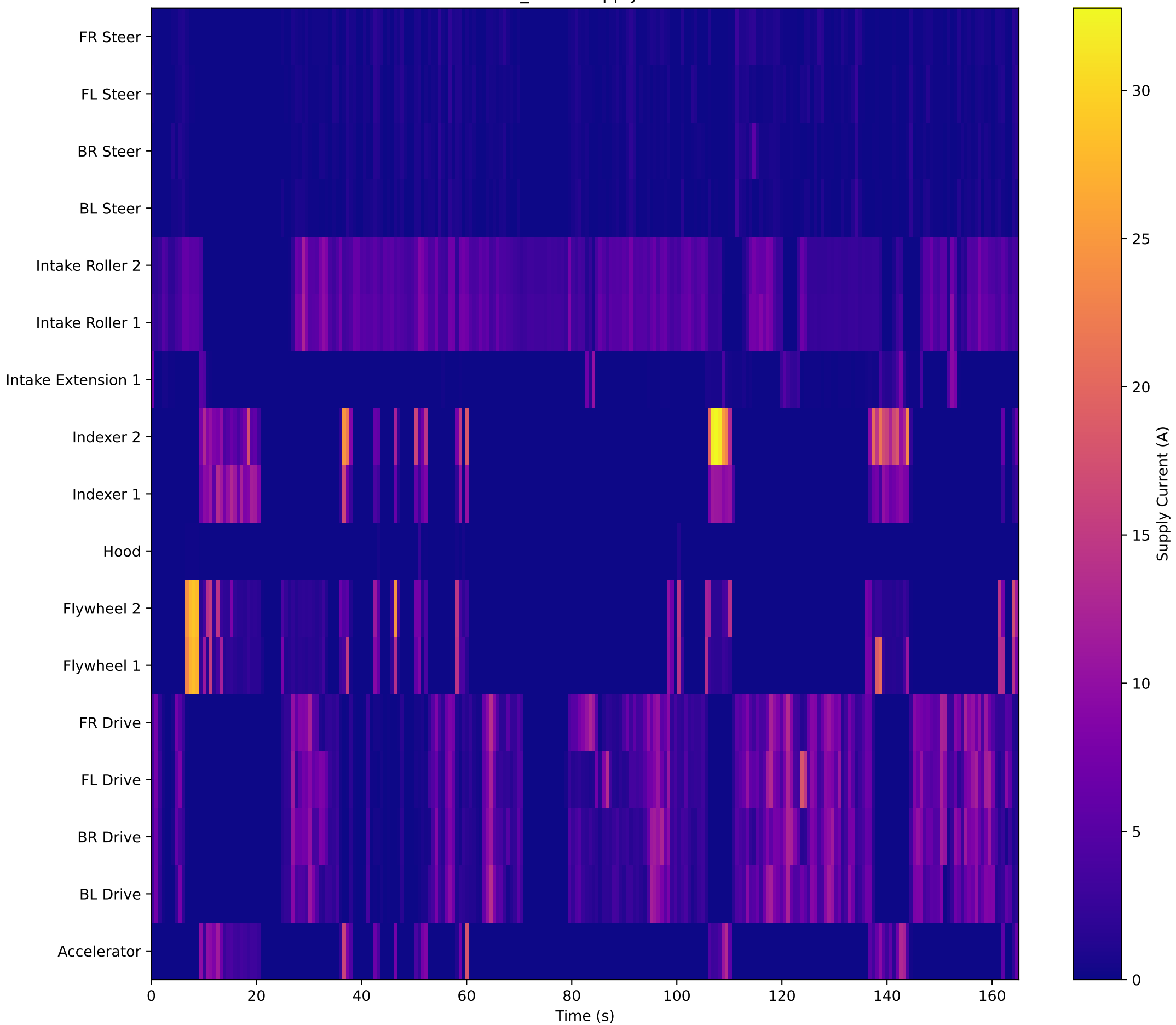
GACOL_E8 — Supply Current
