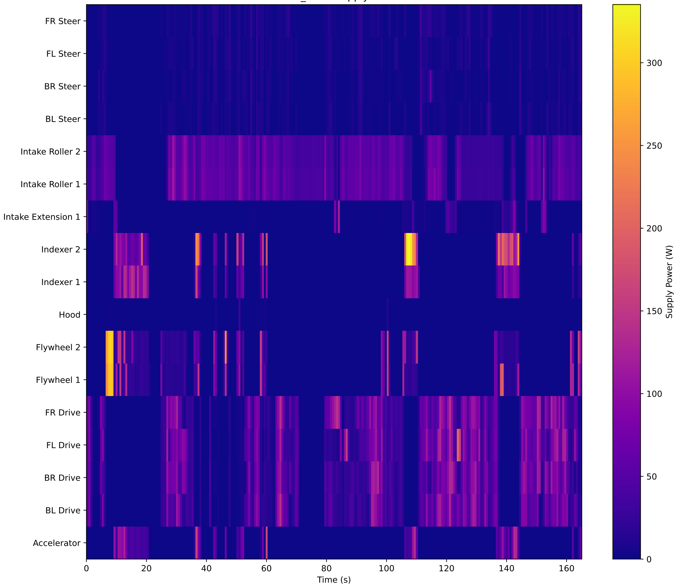
GACOL_E8 — Supply Power
