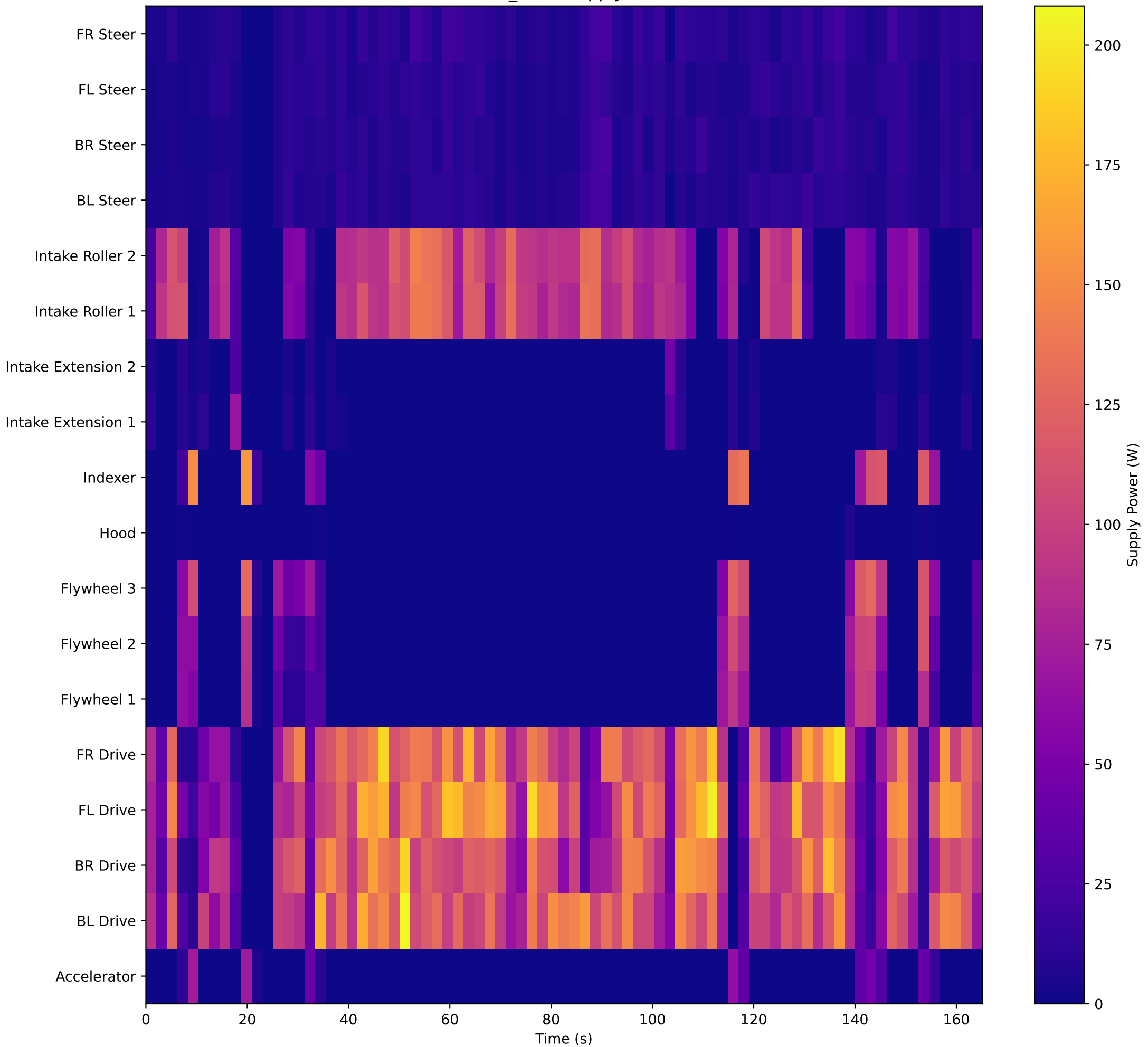
GACMP_E5 — Supply Power
