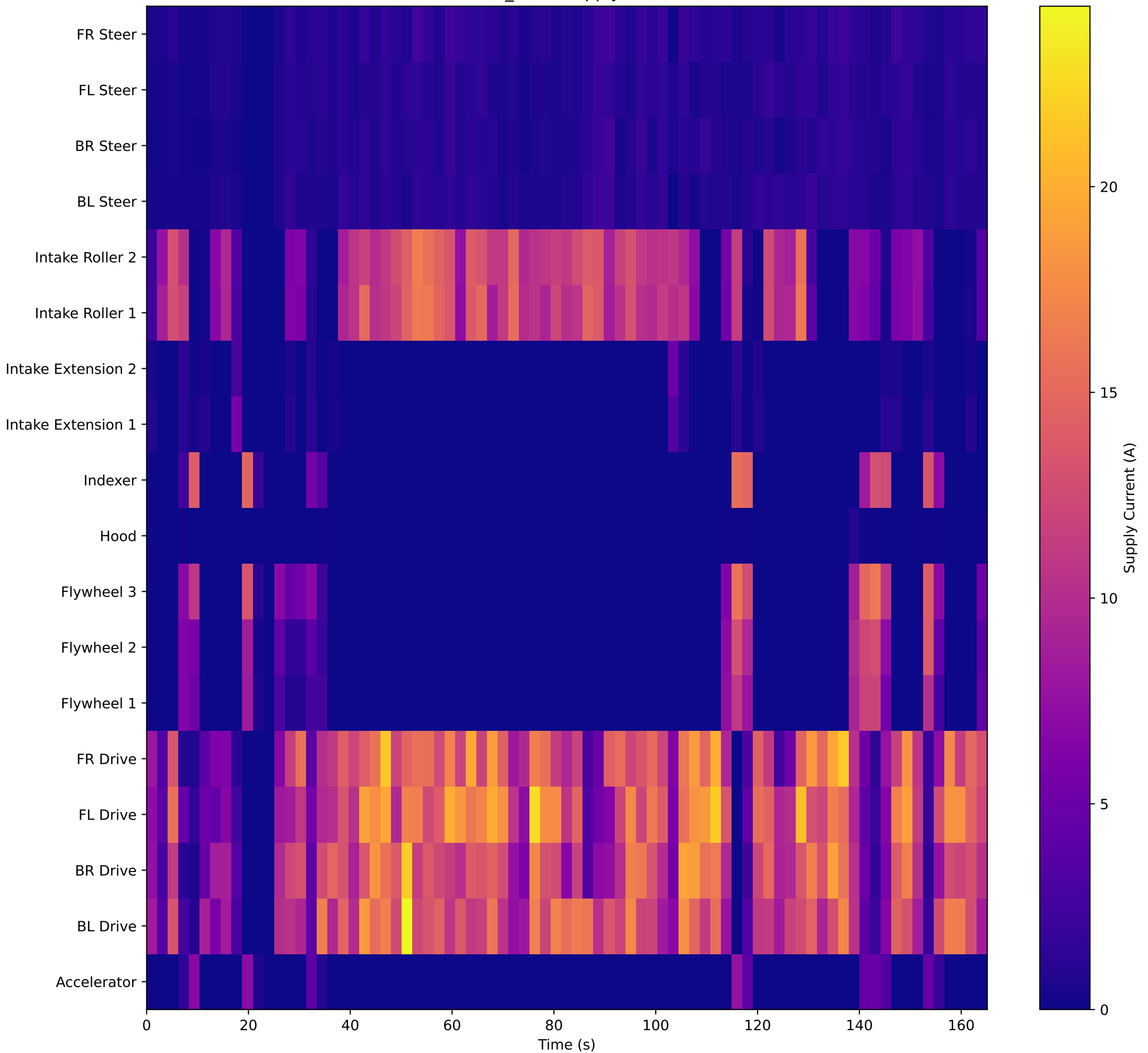
GACMP_E5 — Supply Current
