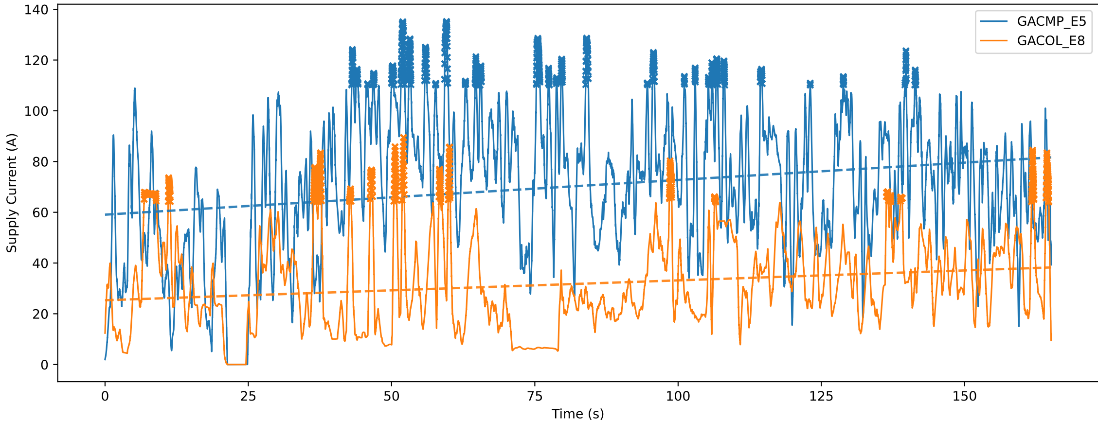
Match Comparison — Supply Current (Robot Total)
