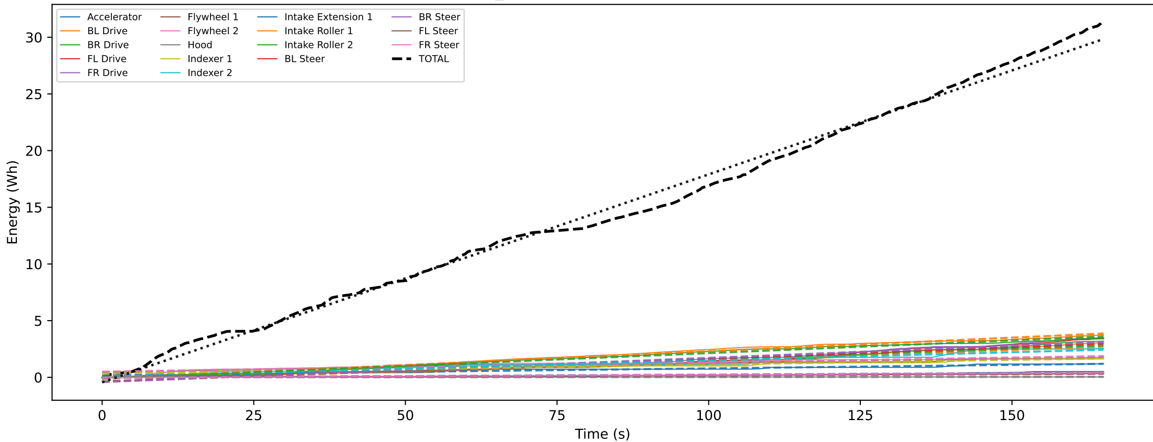
GACOL_E8 — Cumulative Supply Energy
