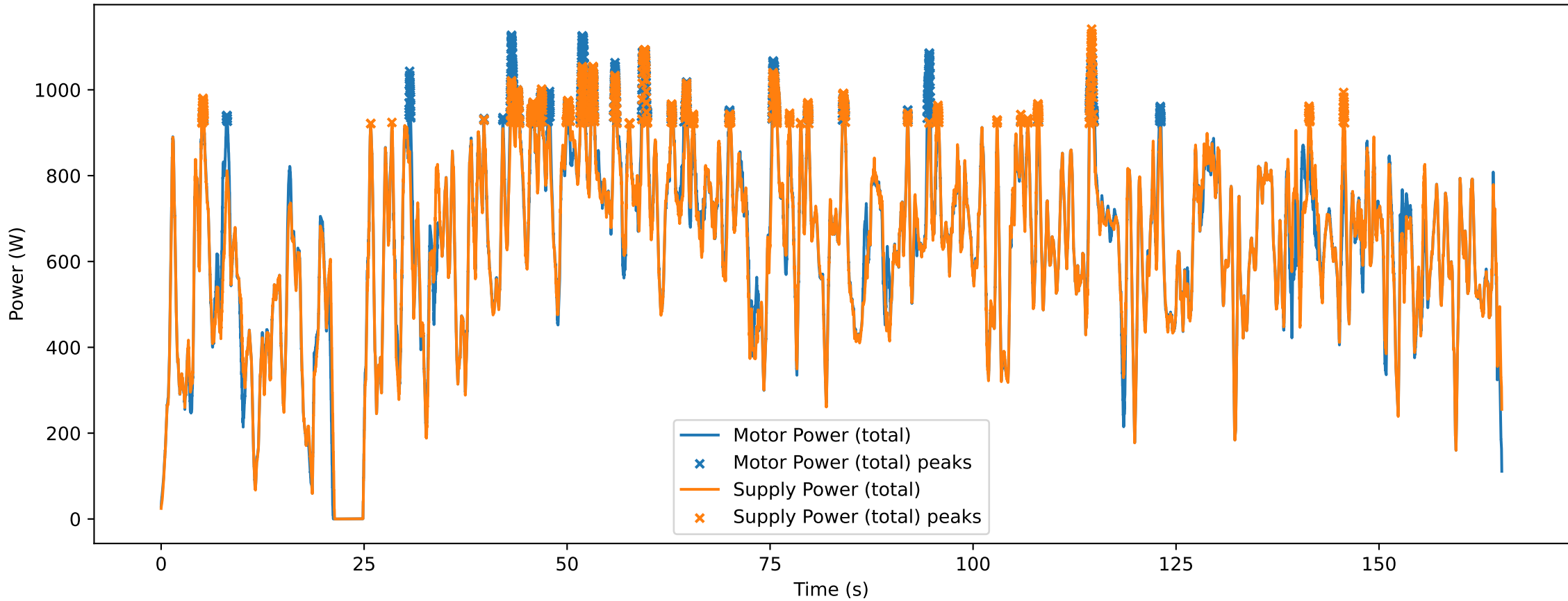
GACMP_E5 — Total Robot Power
