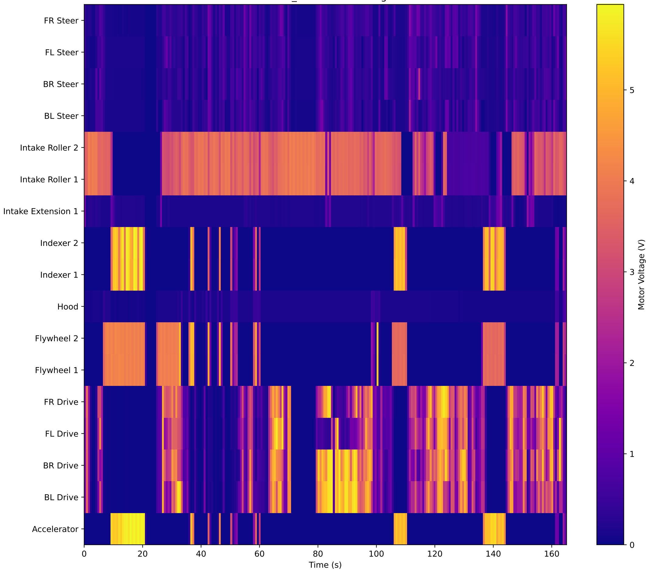
GACOL_E8 — Motor Voltage
