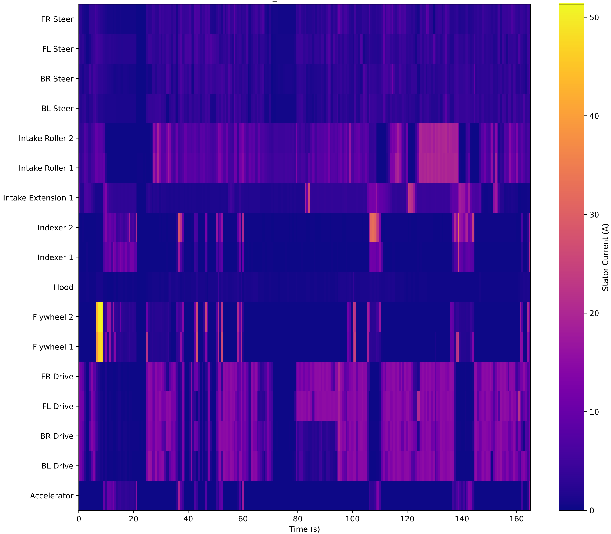
GACOL_E8 — Stator Current
