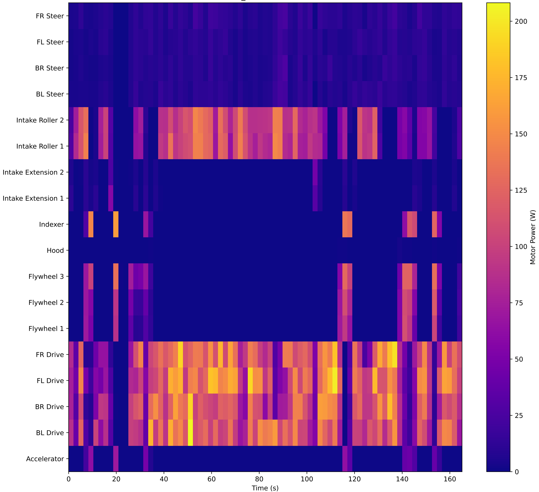
GACMP_E5 — Motor Power
