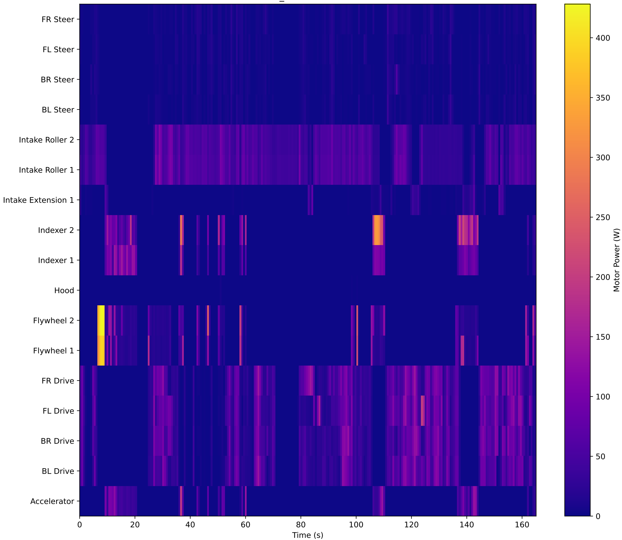
GACOL_E8 — Motor Power
