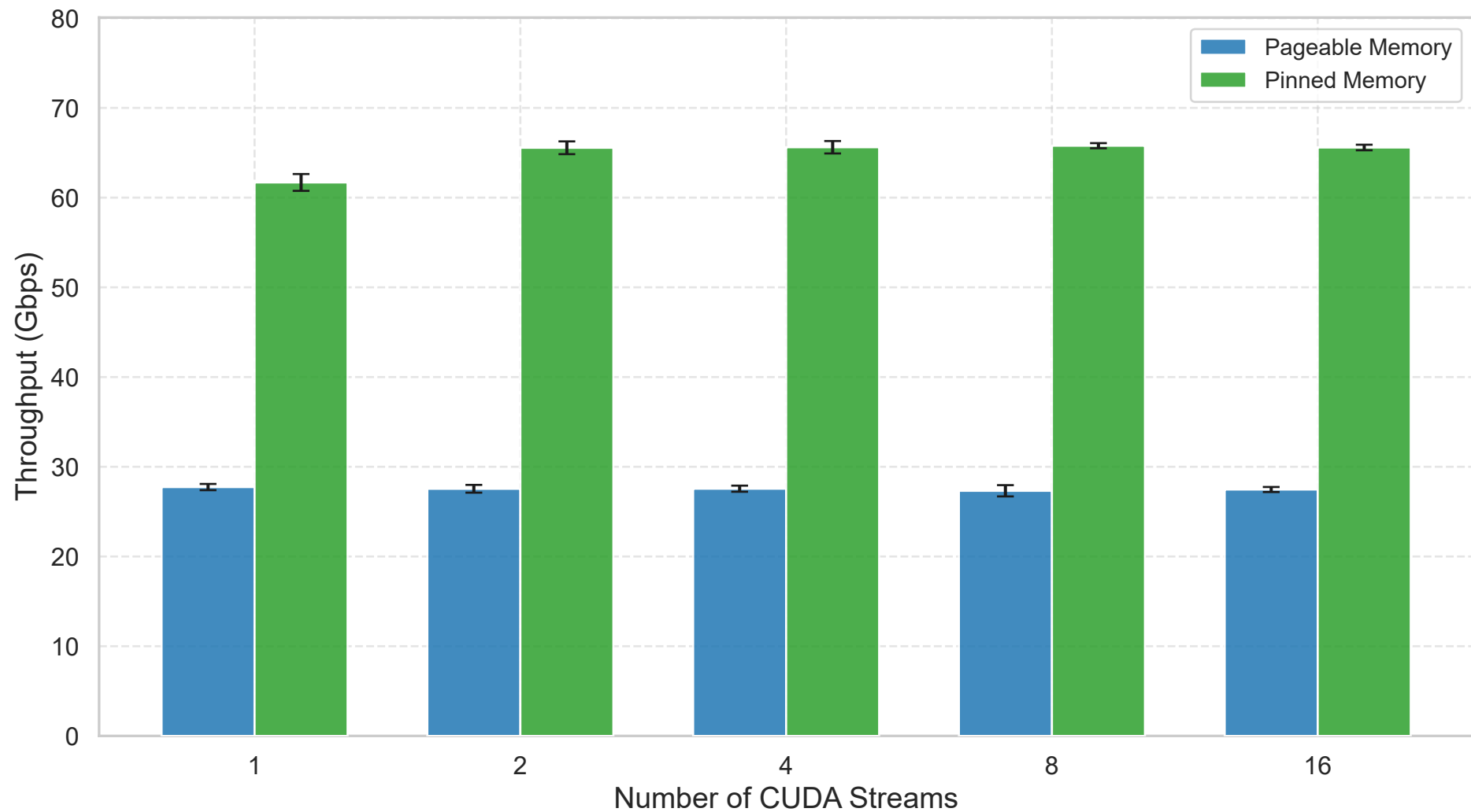
Bidirectional (H2D + D2H) Throughput by Number of Streams
