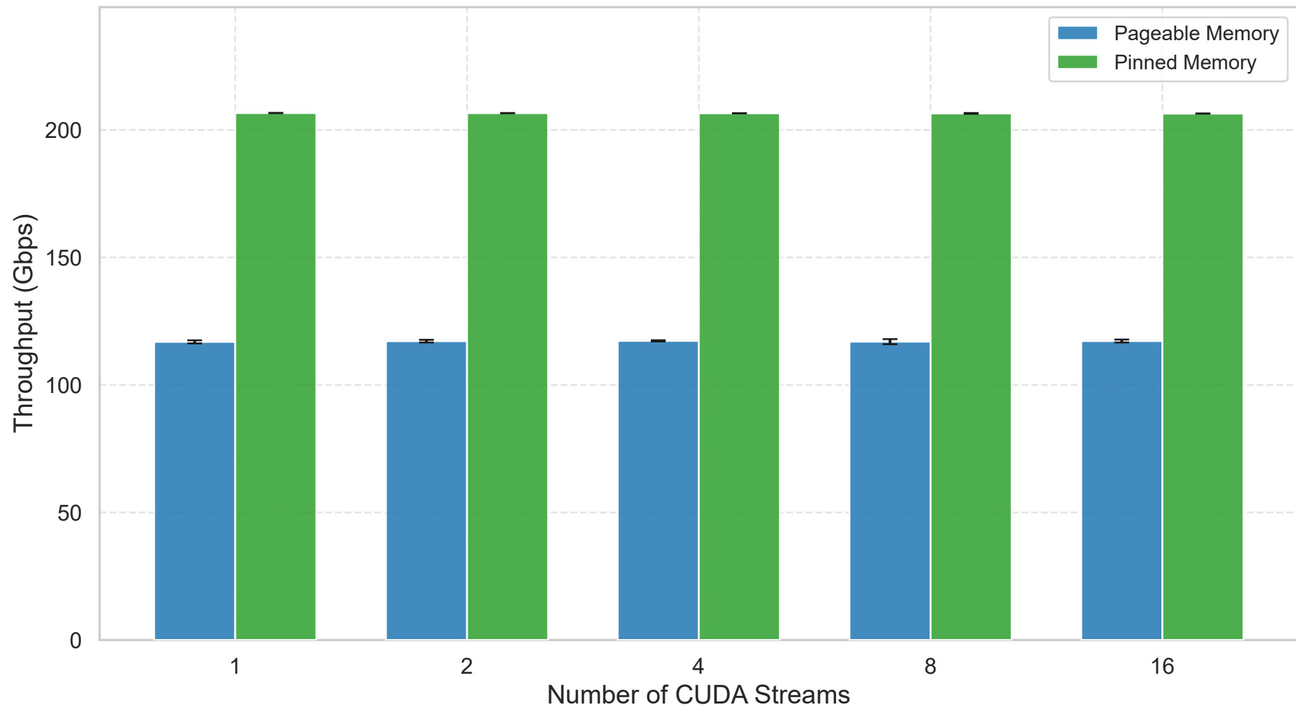
Host-to-Device (H2D) Throughput by Number of Streams
