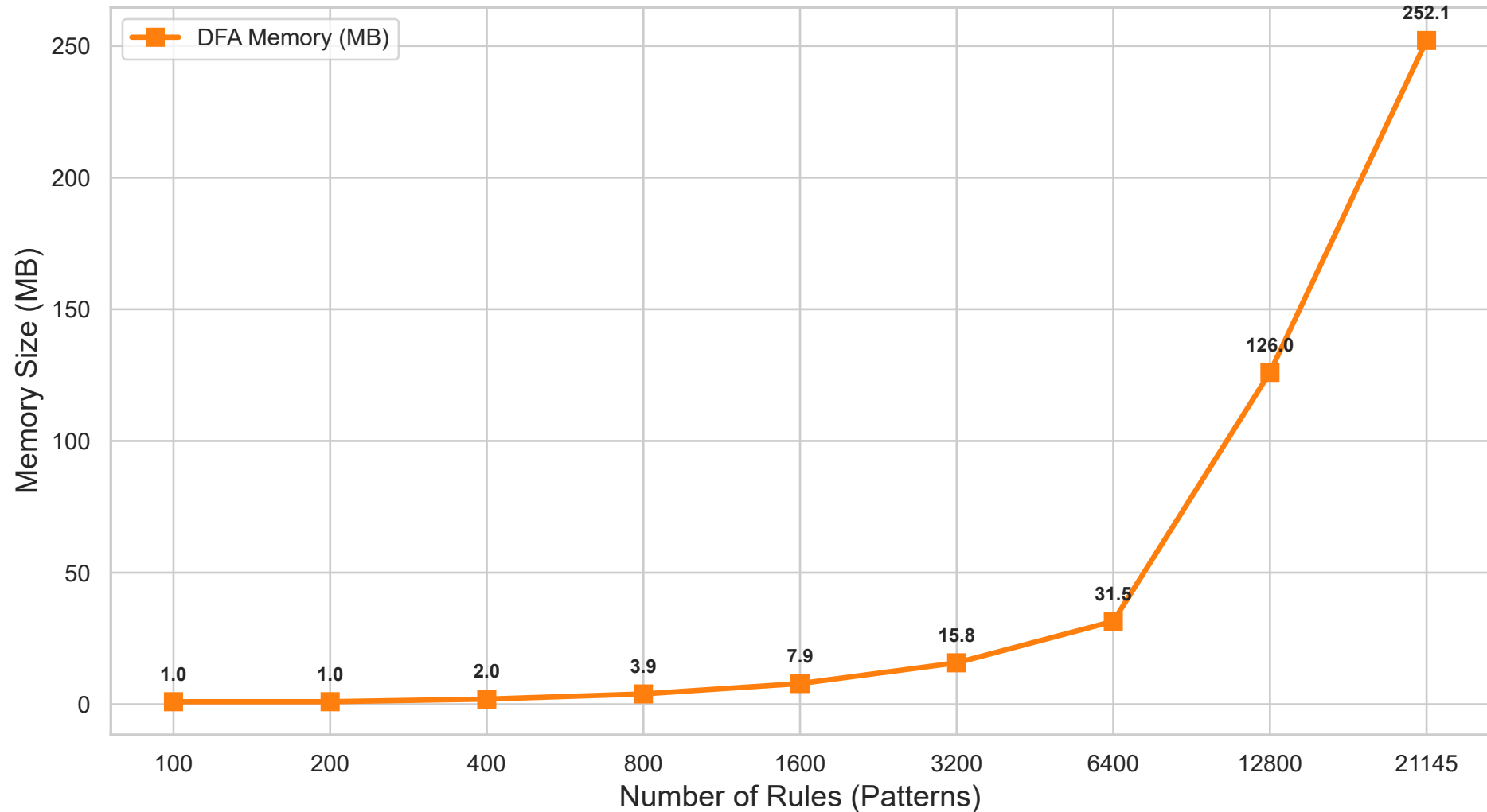
CPU DFA Memory Scaling with Rule Count
