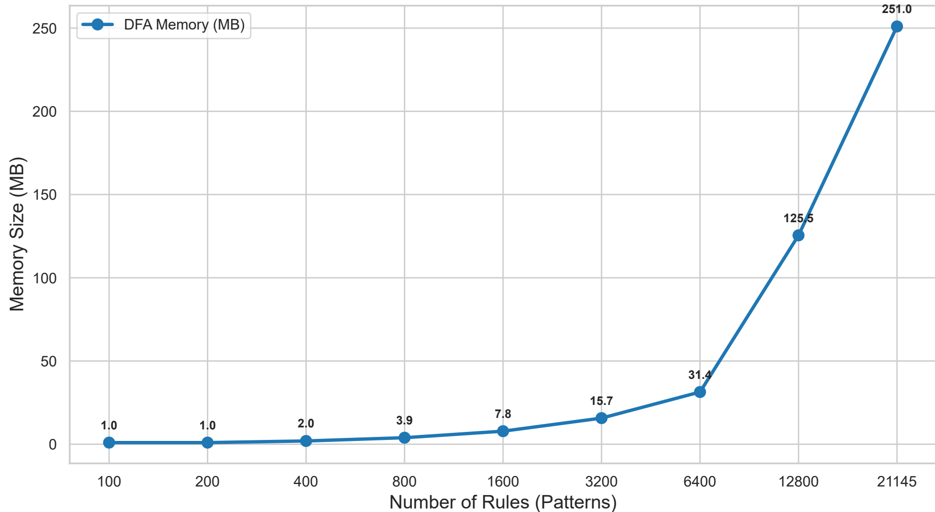
GPU DFA Memory Scaling with Rule Count
