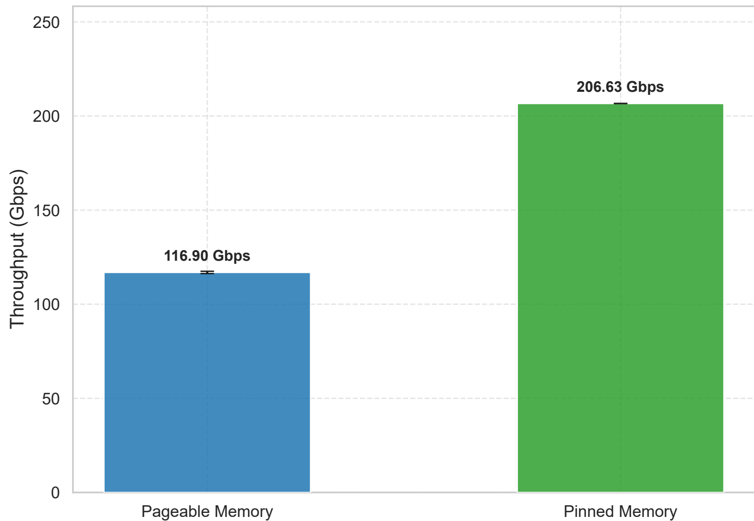
Host-to-Device Transfer Throughput: Pageable vs. Pinned Memory
