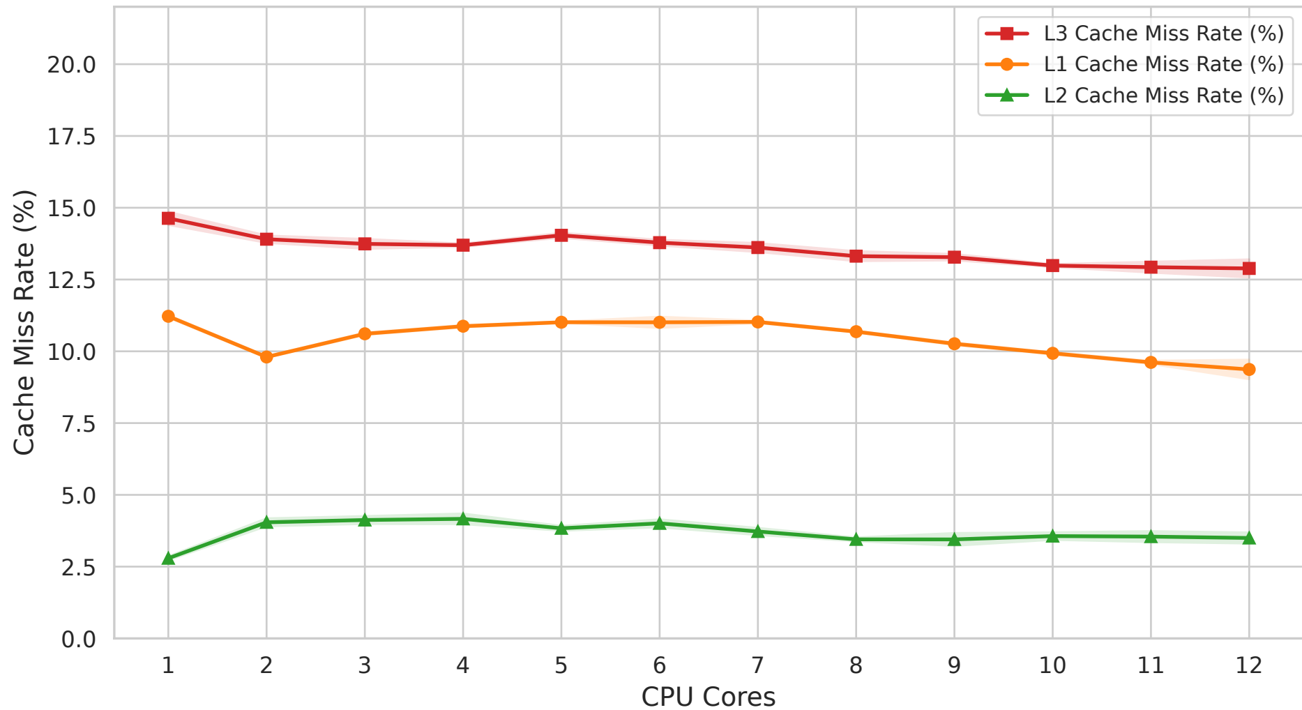
Cache Miss Rates Across Core Scaling
