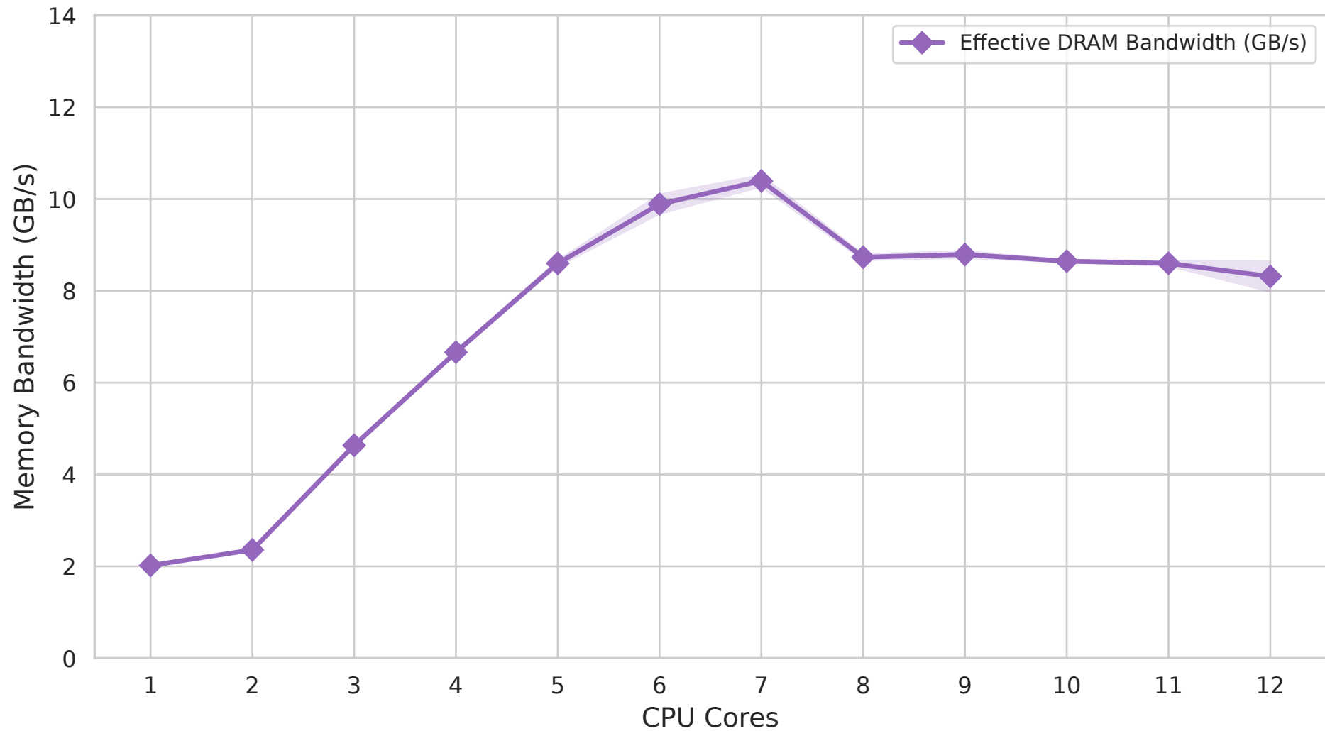
Memory Bus Utilization
