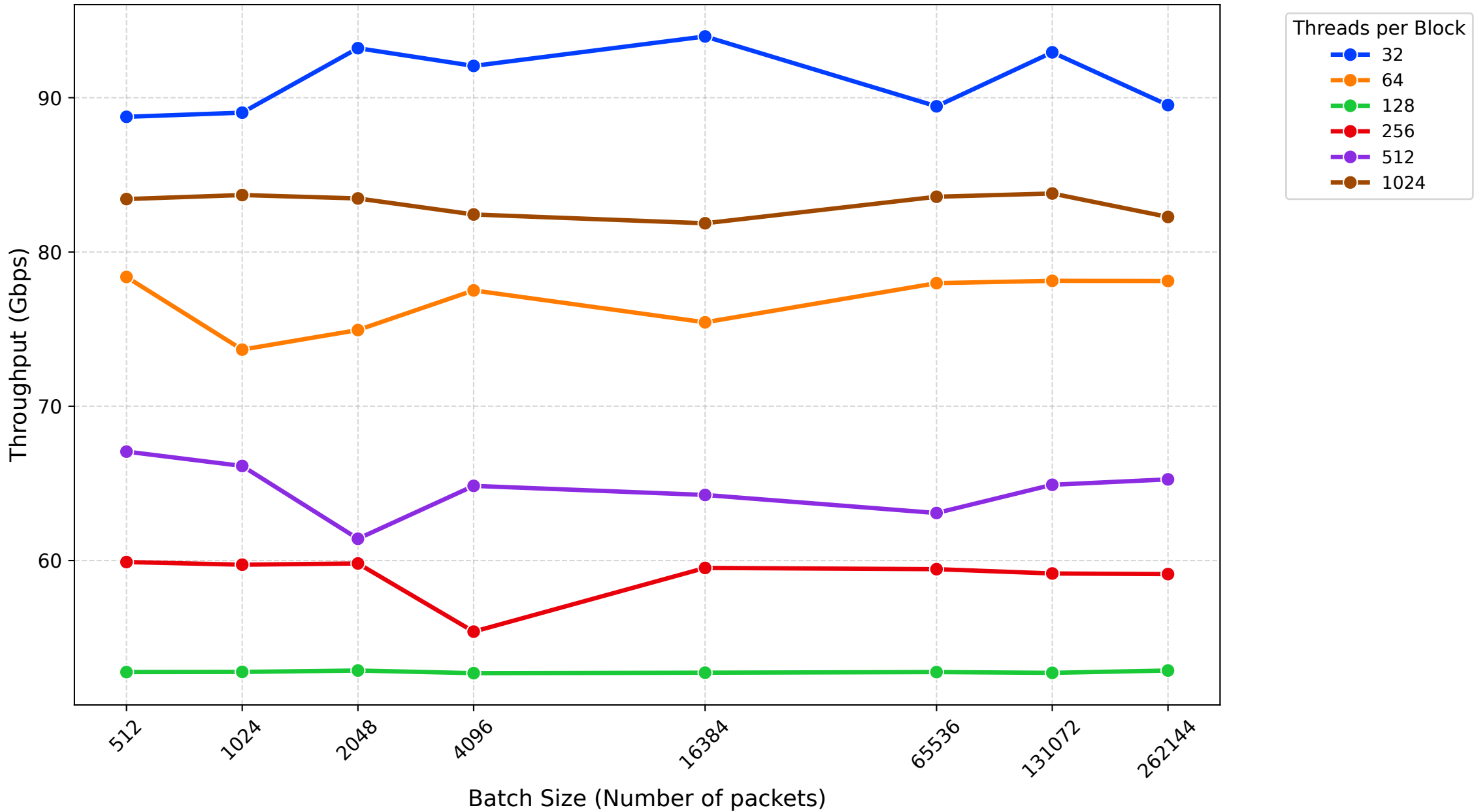
GPU Async Performance: Throughput Scalability vs. Batch Size
