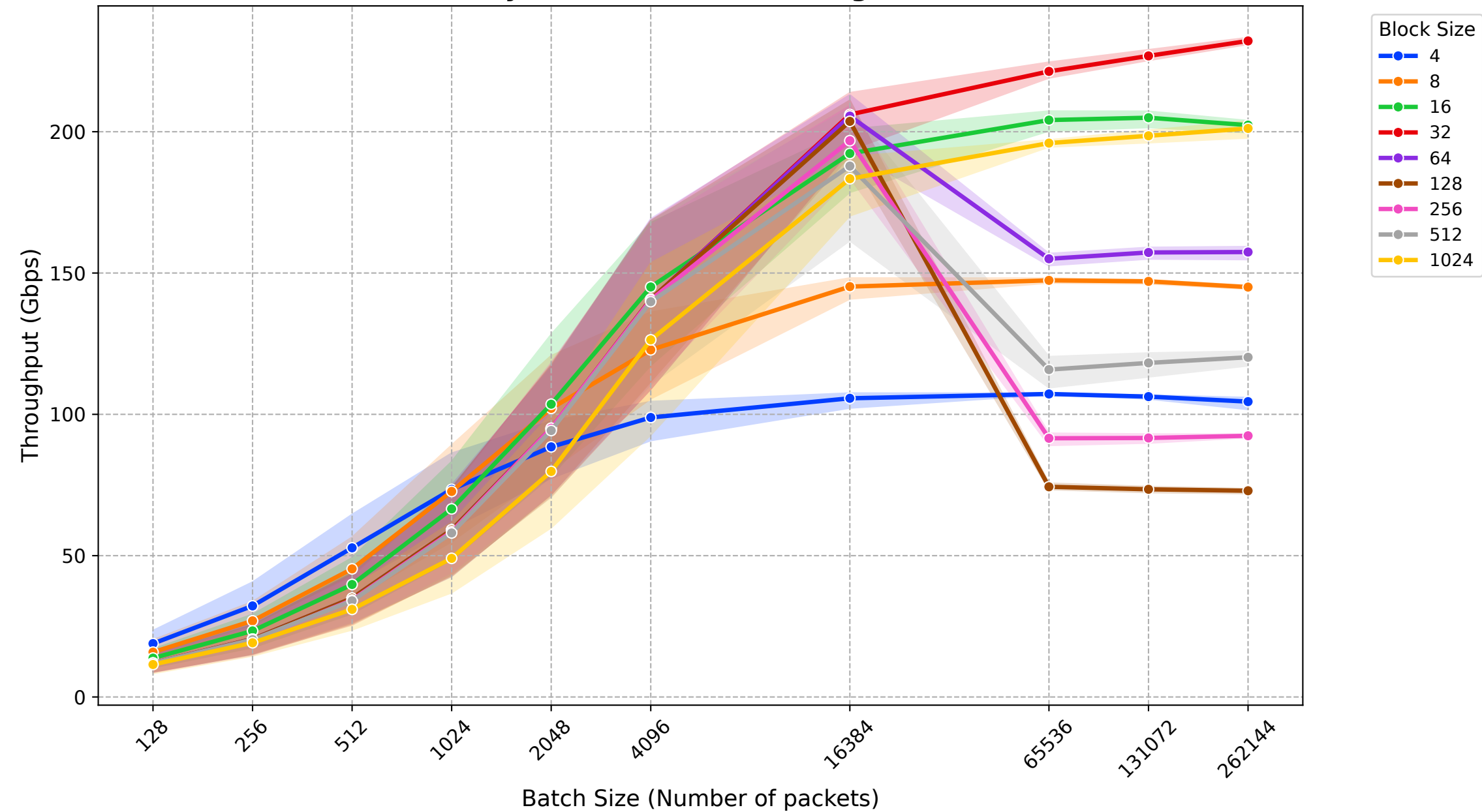
GPU Async Performance Scaling (95% CI)
