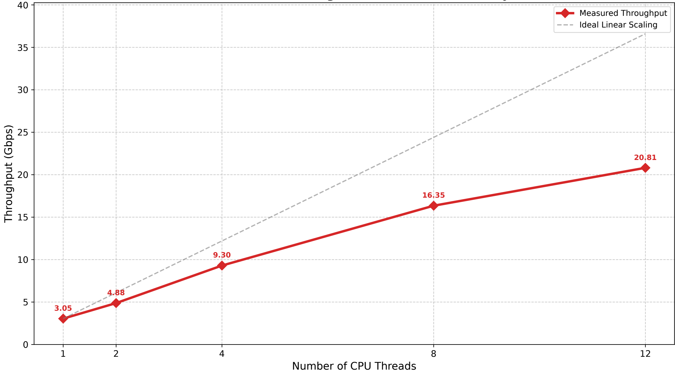
CPU Multi-threading Performance & Efficiency
