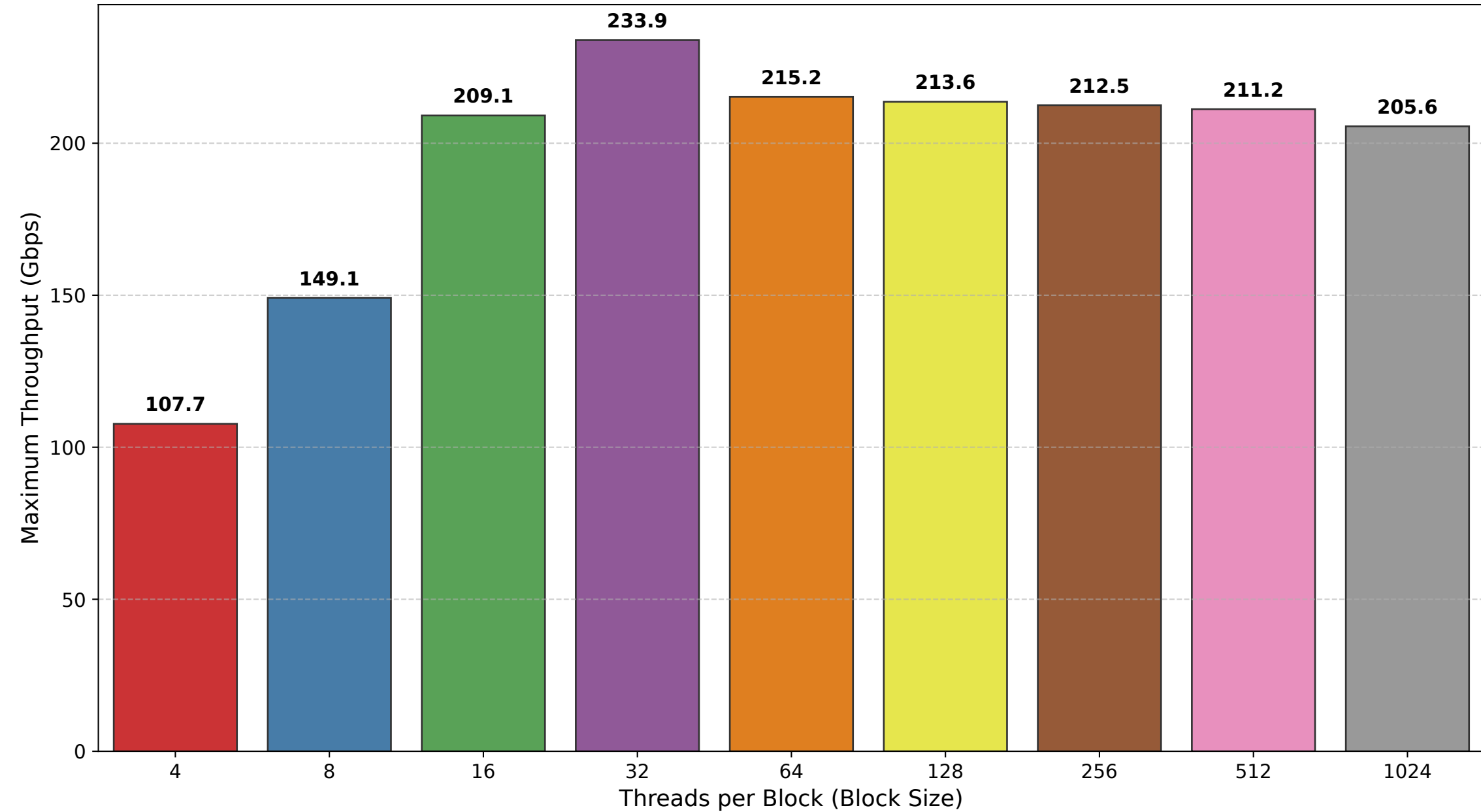
Impact of Block Size on GPU Throughput
