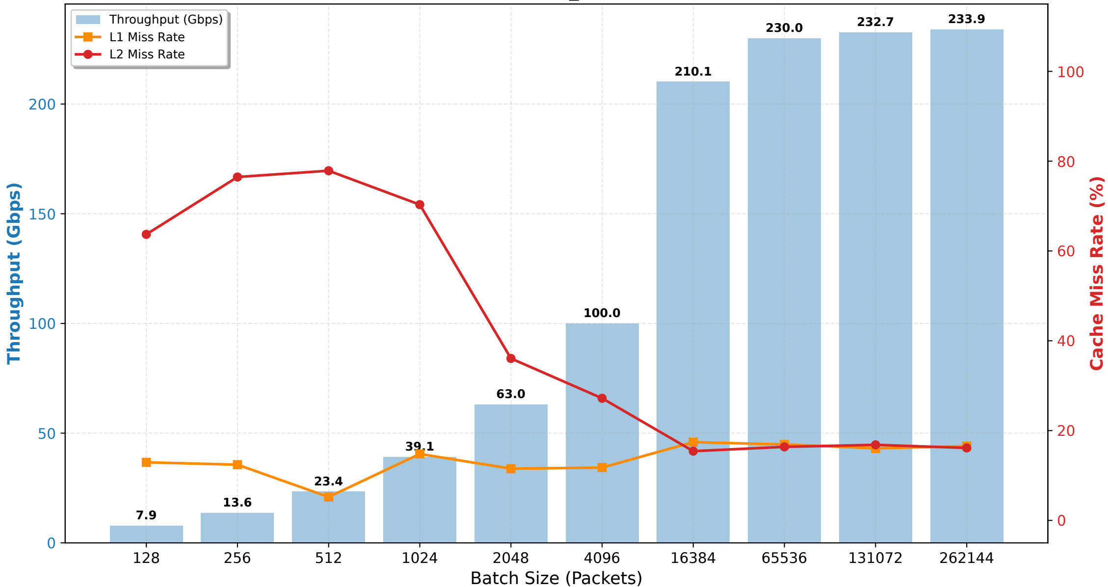
Performance vs. Memory Efficiency (Batch Size) Block: 32, N_Buffer: 3
