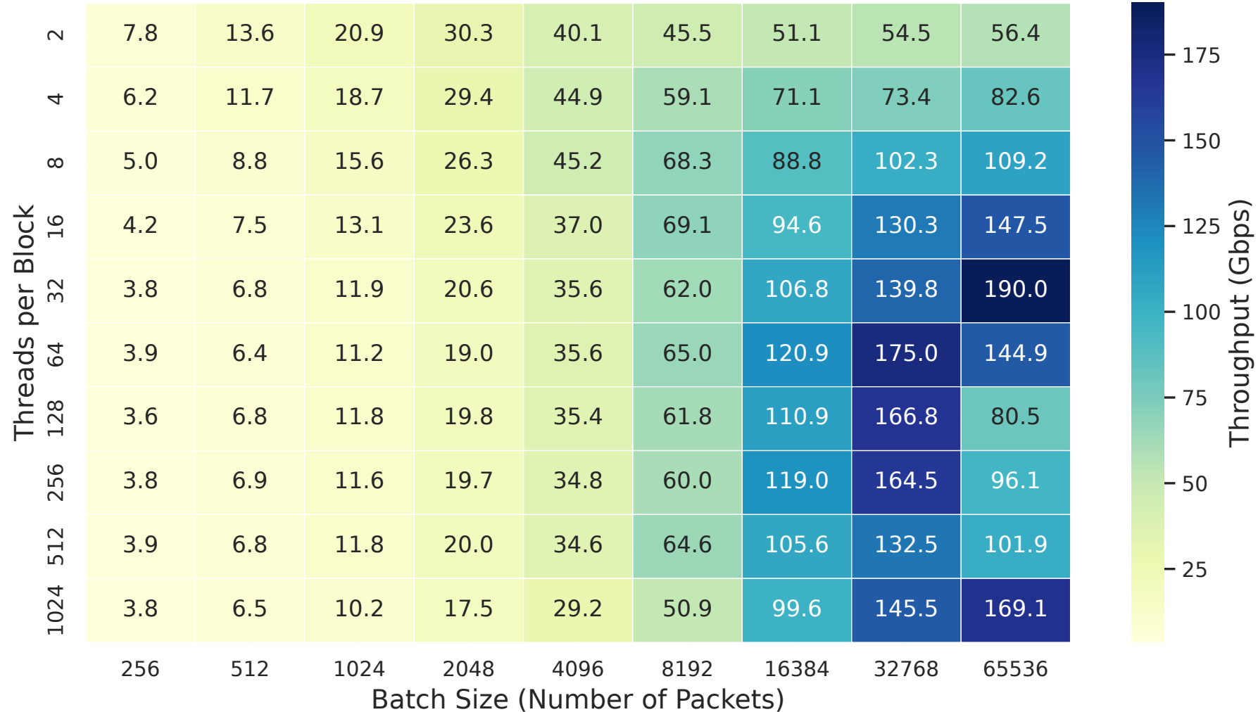
GPU In-Memory Aho-Corasick Throughput Grid Search
