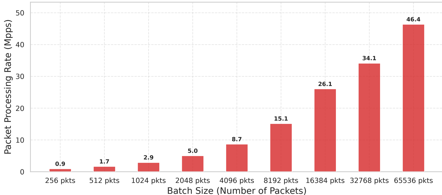
GPU Processing Rate (Mpps) by Batch Size (Packets)
