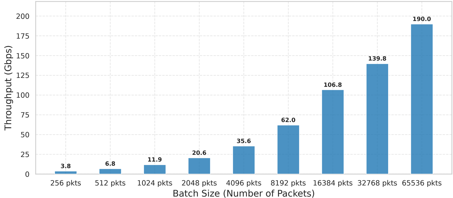
GPU Throughput scaling by Batch Size (Packets)
