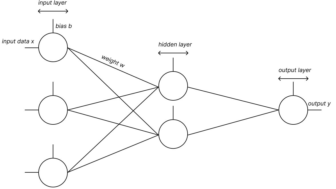
Figure 4: Example of a neural network. Figure heavily inspired by a figure from [48].
