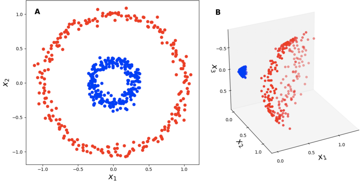
Figure 2: Input features in 2D where they aren't separable by a 2D hyperplane (a line) and in 3D, where they are separable by a 3D hyperplane (a plane) [20].
