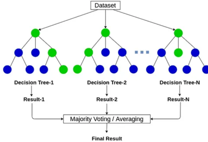
Figure 3: High level overview of Random Forests: The predictions of the trees are transformed into one prediction via majority voting or averaging [25].
