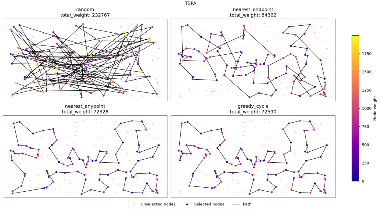
Figure 1: Best solutions for TSPA
