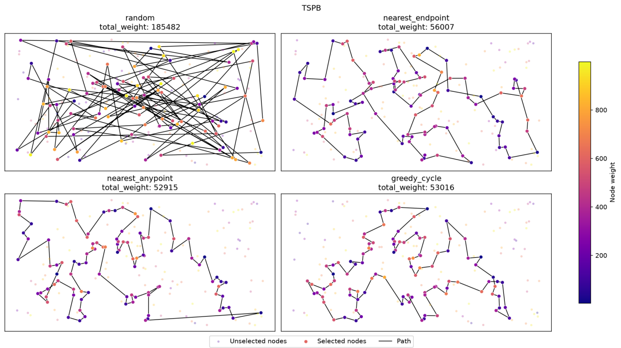
Figure 2: Best solutions for TSPB
