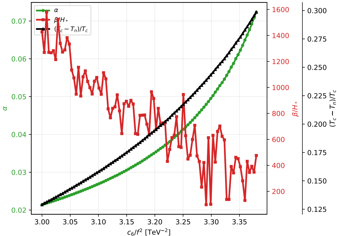
Run 05: pure \phi^6 + \phi^8 scan: c_8/f^4 [TeV ^{-4} ]=2, no daisy
