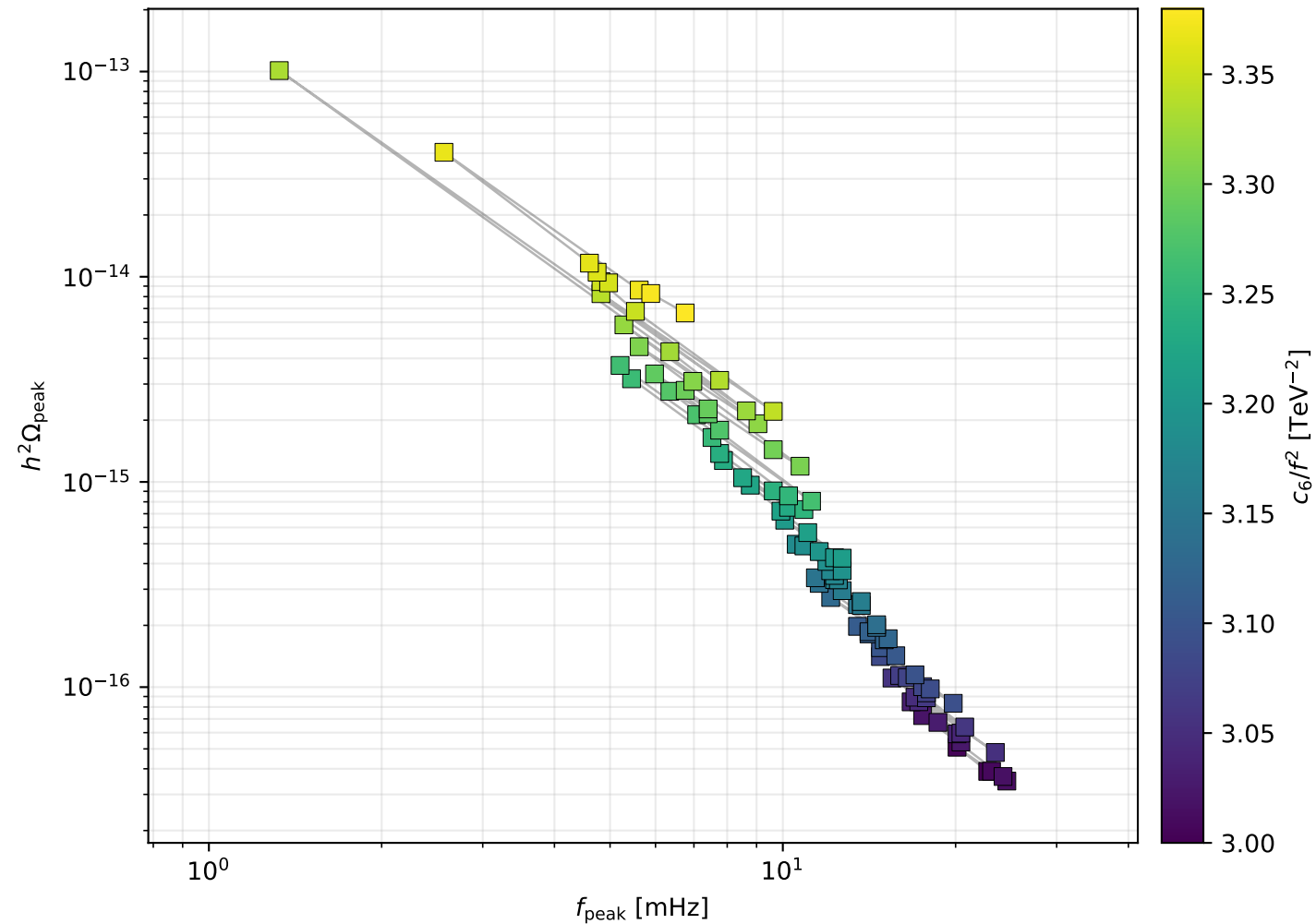
Run 05: pure \phi^6 + \phi^8 scan: peak motion, c_8/f^4 [TeV ^{-4} ]=2, with daisy
