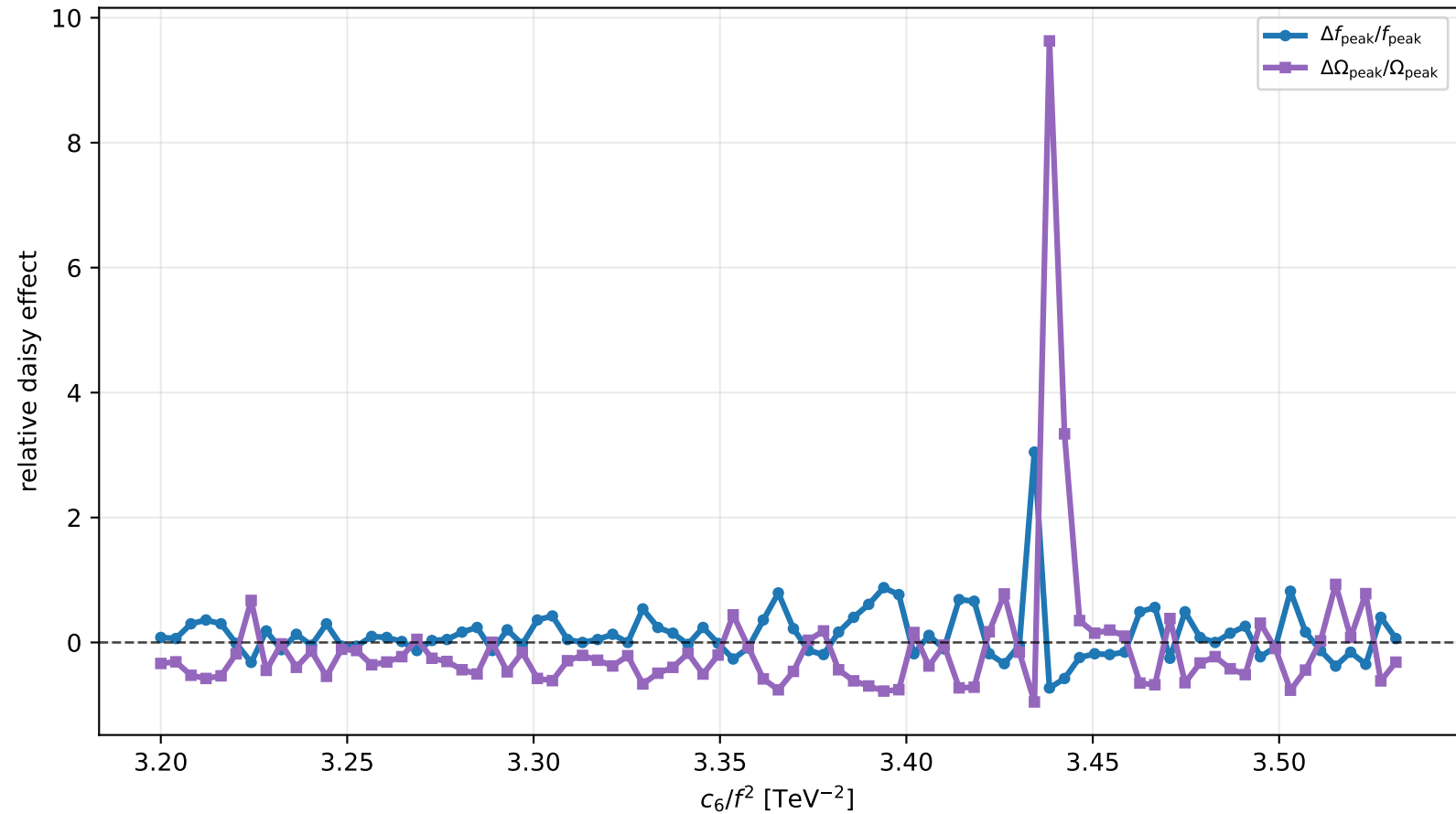
Run 05: pure \phi^6 + \phi^8 scan: relative peak shift, c_8/f^4 [TeV ^{-4} ]=0
