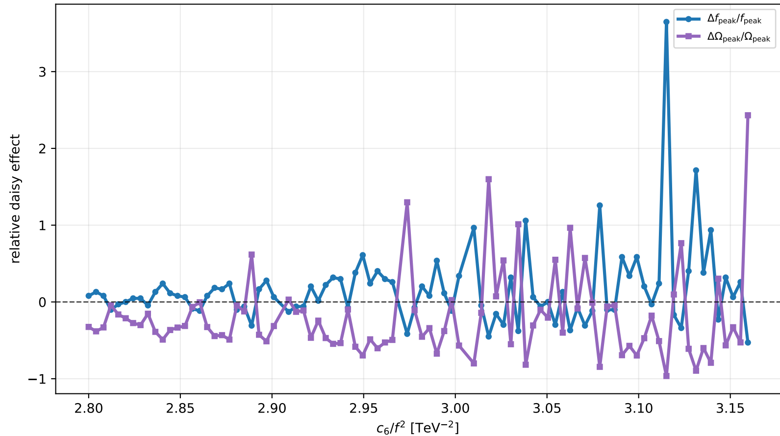
Run 05: pure \phi^6 + \phi^8 scan: relative peak shift, c_8/f^4 [TeV ^{-4} ]=5
