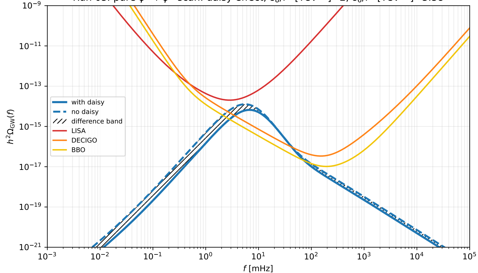
Run 05: pure \phi^6 + \phi^8 scan: daisy effect, c_8/f^4 [TeV ^{-4} ]=2, c_6/f^2 [TeV ^{-2} ]=3.38
