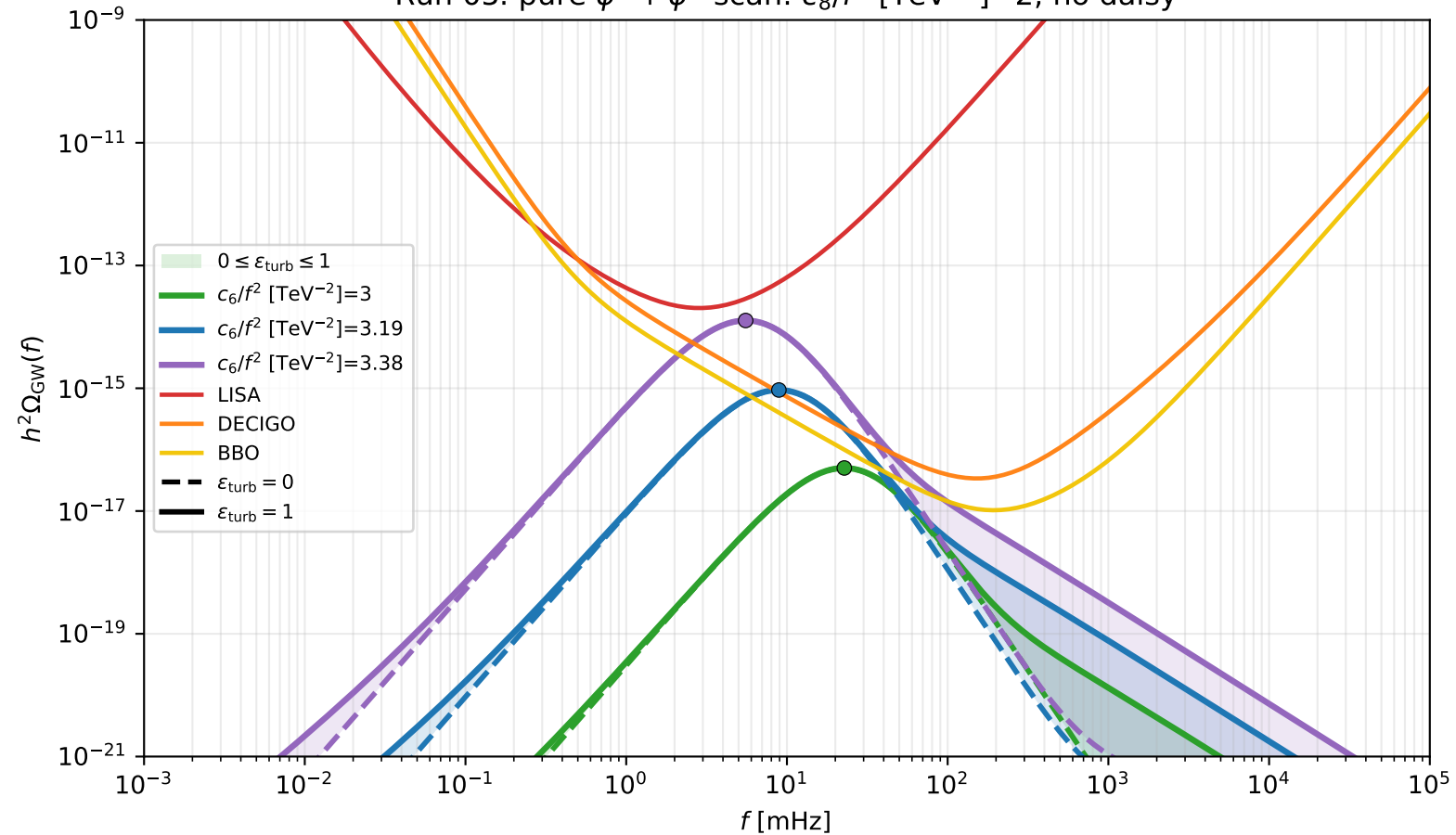
Run 05: pure \phi^6 + \phi^8 scan: c_8/f^4 [TeV ^{-4} ]=2, no daisy
