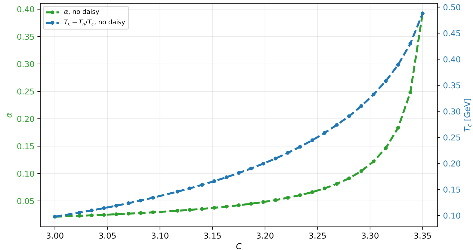
Run 06: combined \phi^6 + \phi^8 + Gláuber scan in C c_8/f^4 = 5 \text{ TeV}^{-4} , c_6/f^2 = 1 \text{ TeV}^{-2} , \Lambda = 1000 \text{ GeV} , f = 1000 \text{ GeV}
