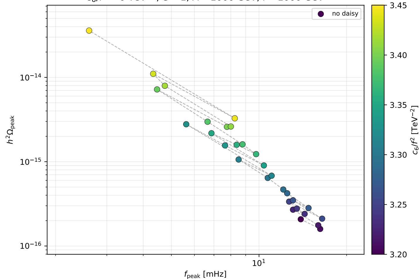
Run 07: combined \phi^6 + \phi^8 + Gláuber scan in c_6/f^2 : peak motion c_8/f^4 = 0 \text{ TeV}^{-4} , C = 1 , \Lambda = 1000 \text{ GeV} , f = 1000 \text{ GeV}
