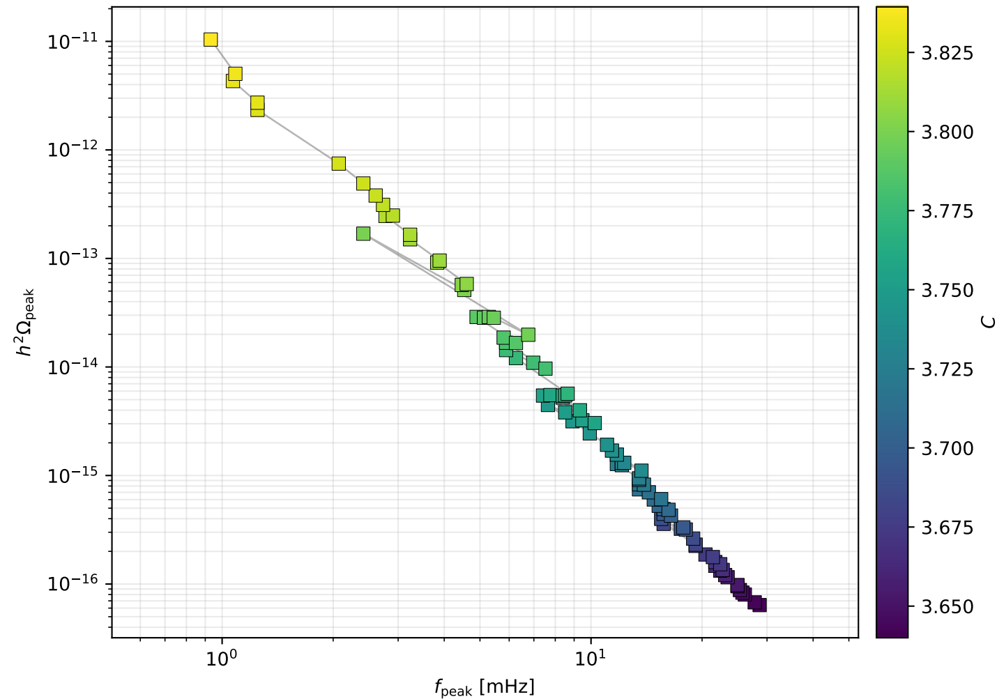
Run 03: pure Gláuber C scan: peak motion, \Lambda [GeV]=1000, with daisy
