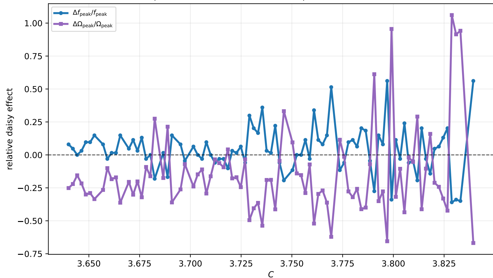
Run 03: pure Gláuber C scan: relative peak shift, \Lambda [GeV]=1000
