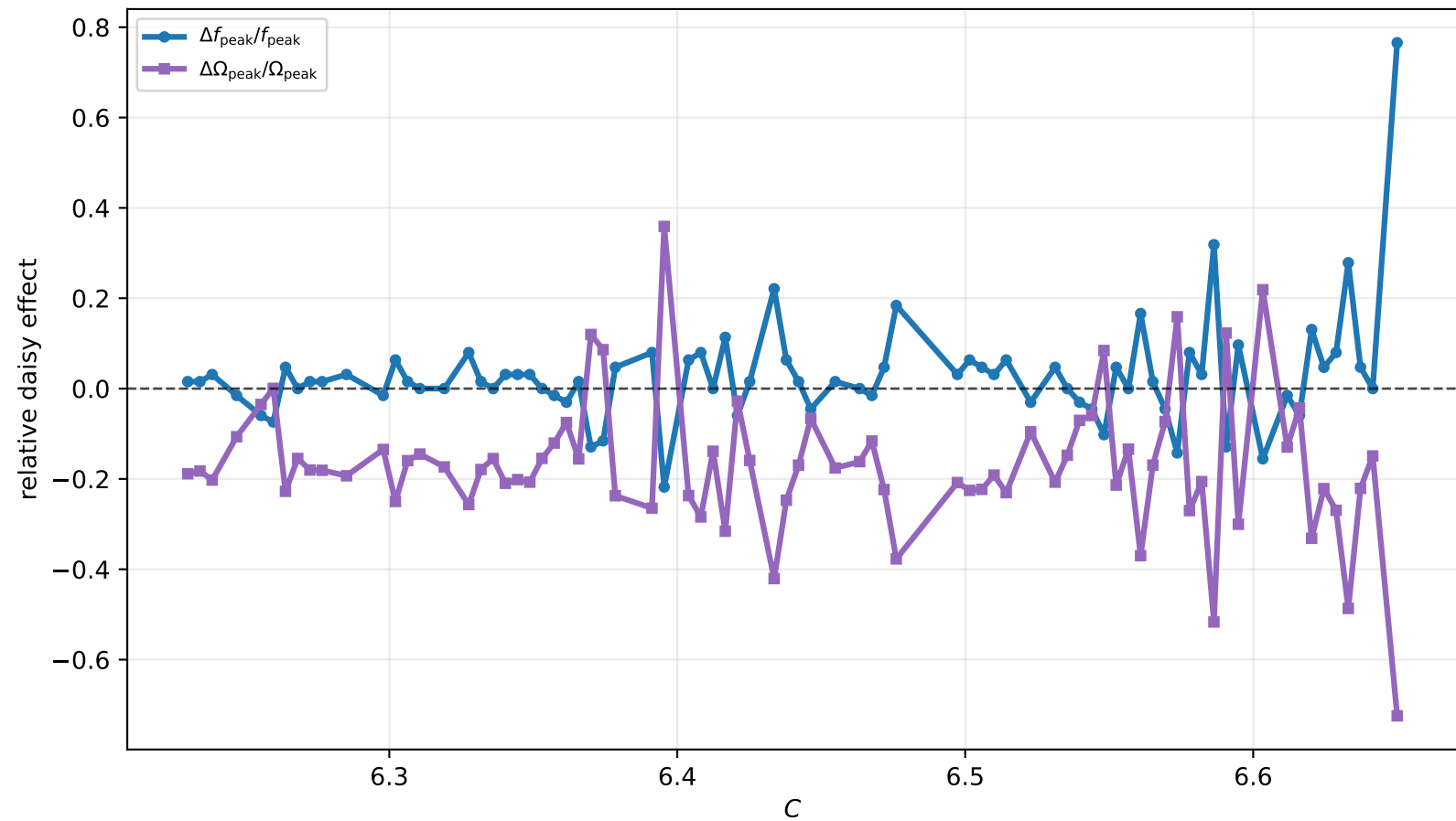
Run 03: pure Gláuber C scan: relative peak shift, \Lambda [GeV]=2000
