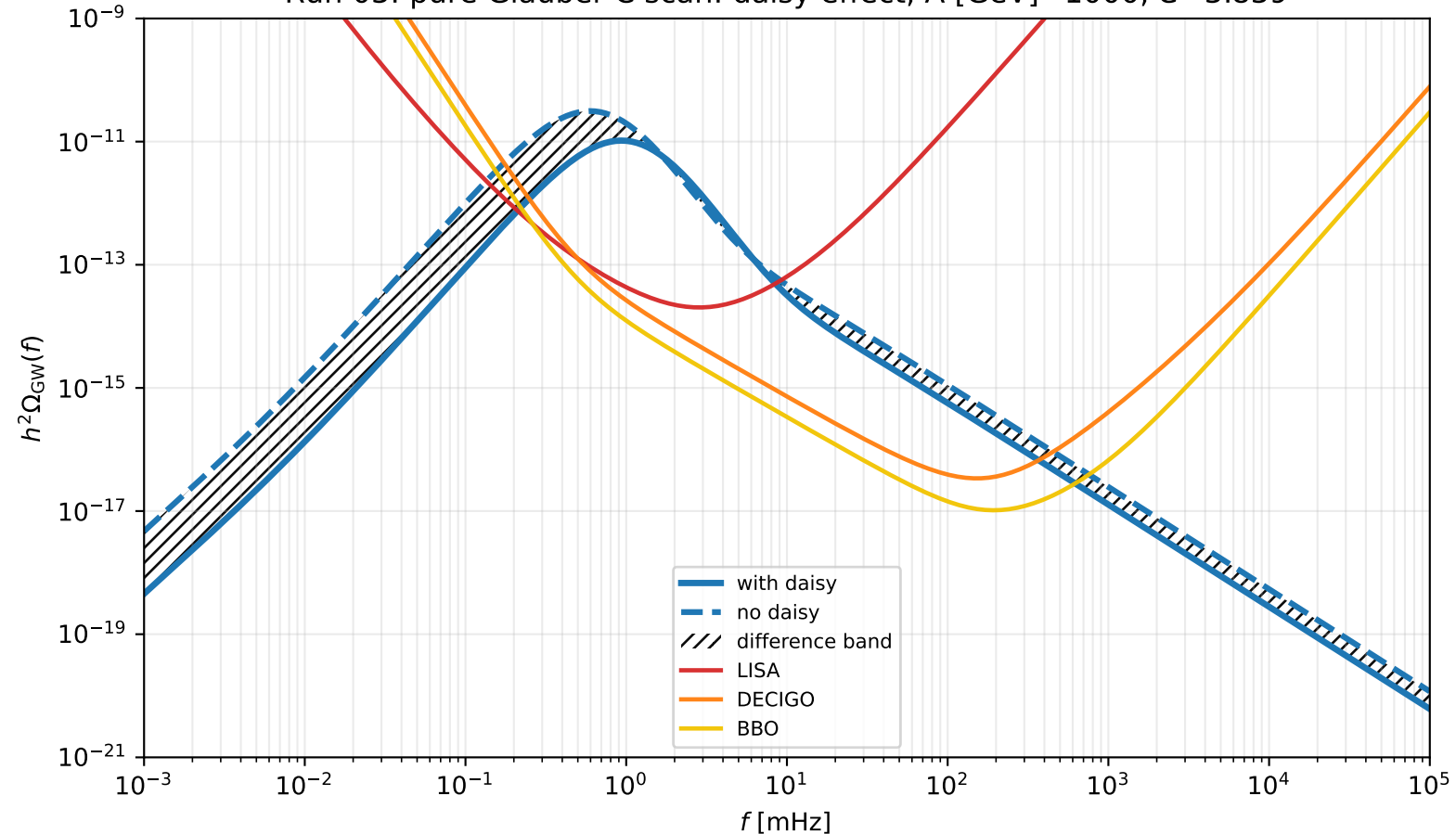
Run 03: pure Gláuber C scan: daisy effect, \Lambda [GeV]=1000, C=3.839
