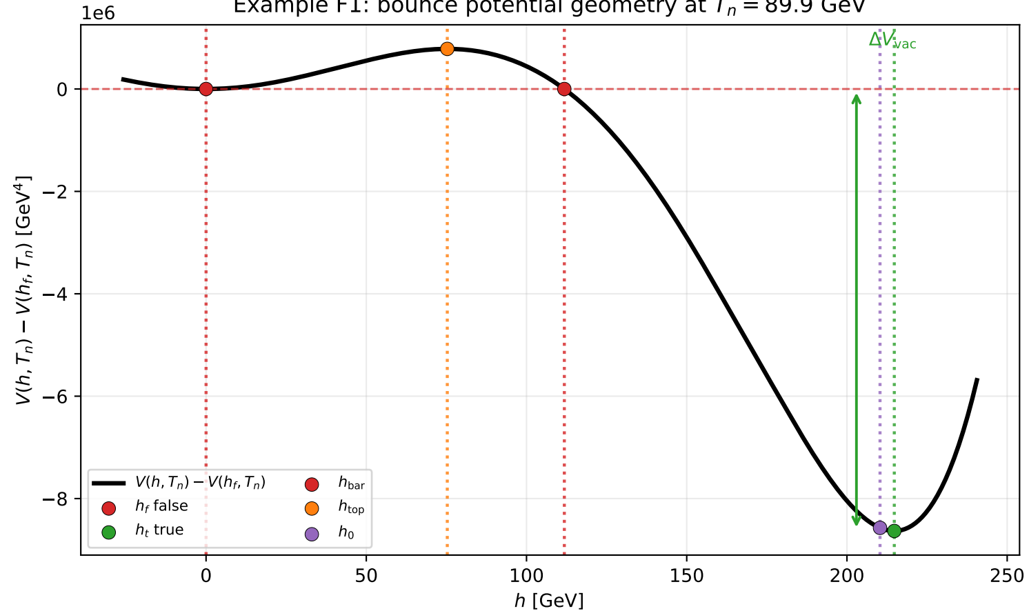
Example F1: bounce potential geometry at T_n = 89.9 GeV
