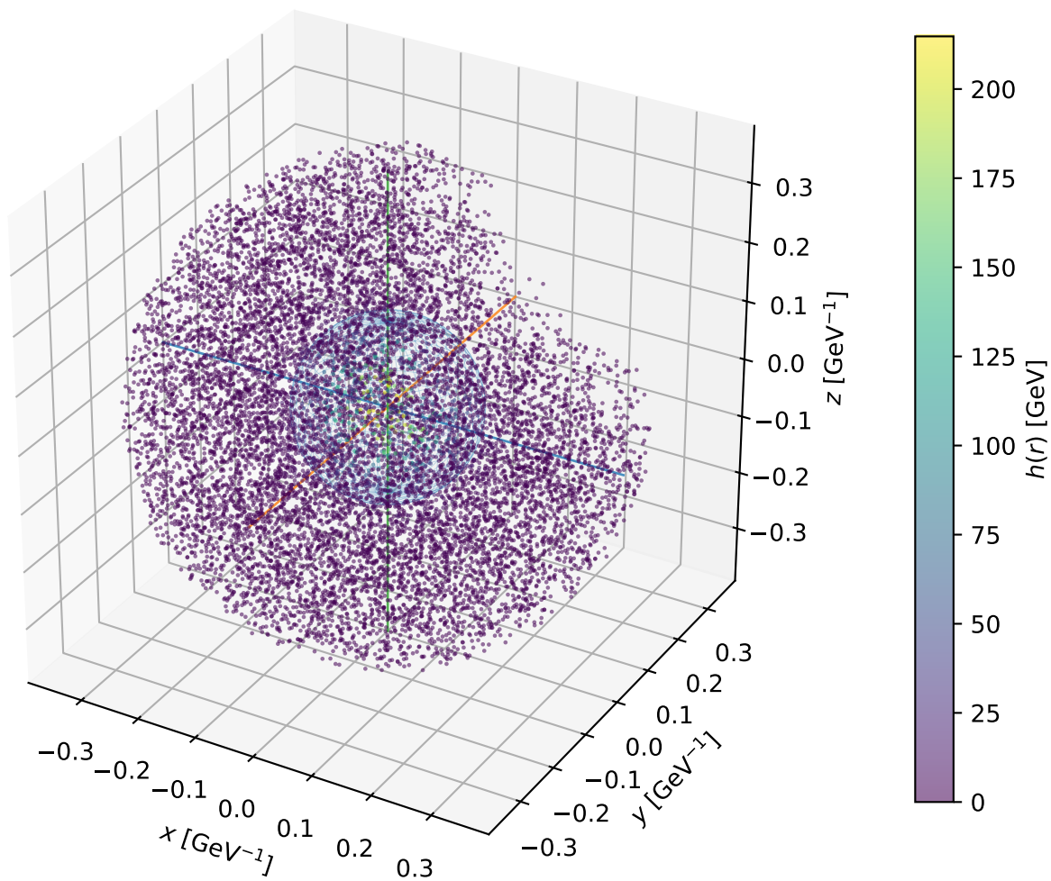
Example F5: 3D bubble profile at T_n = 89.9 GeV
