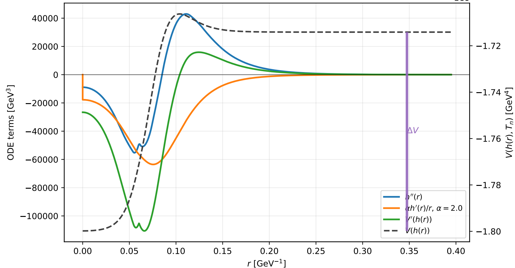
Example F7: bounce equation terms at T_n = 89.9 GeV
