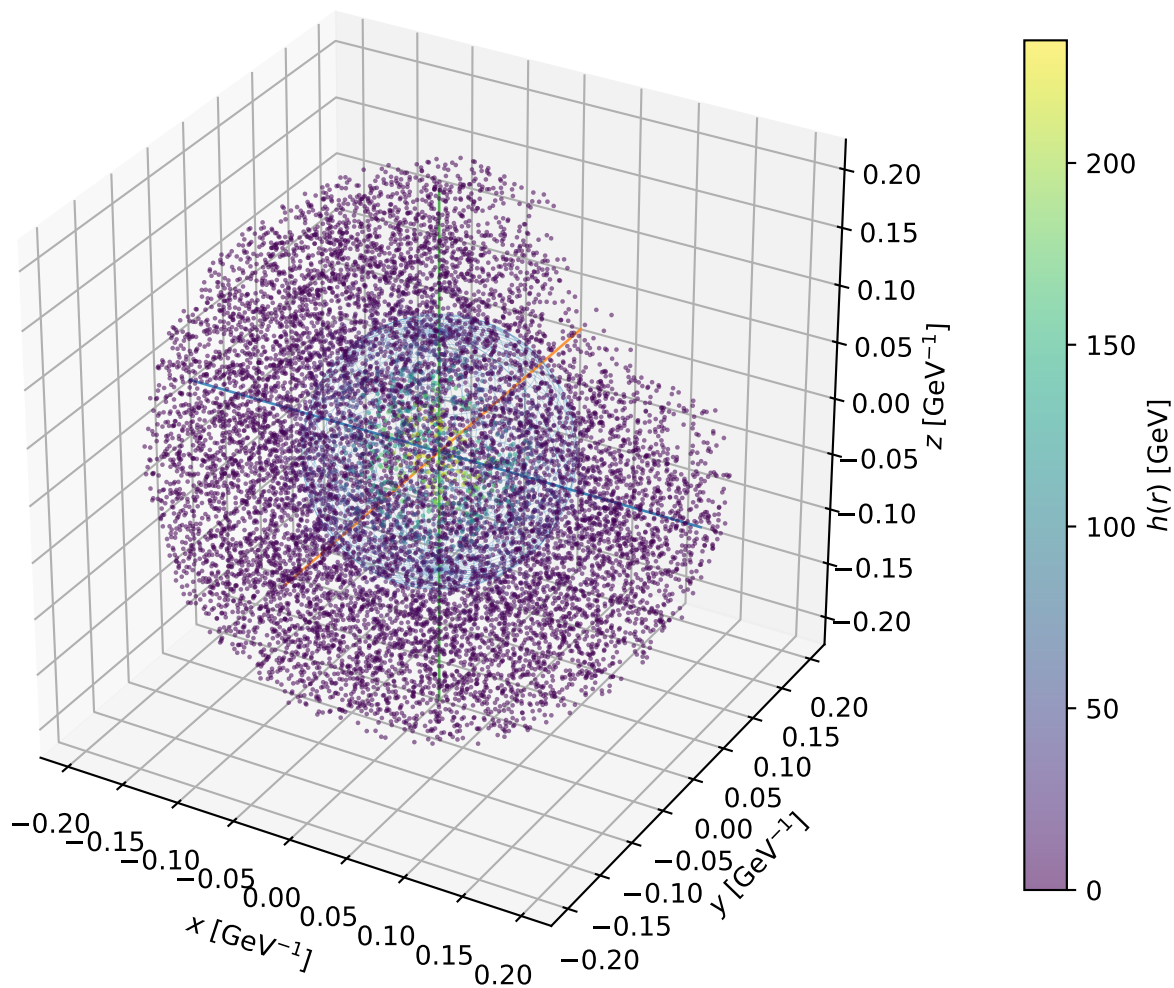
Example F5: 3D bubble profile at T_n = 70.64 GeV
