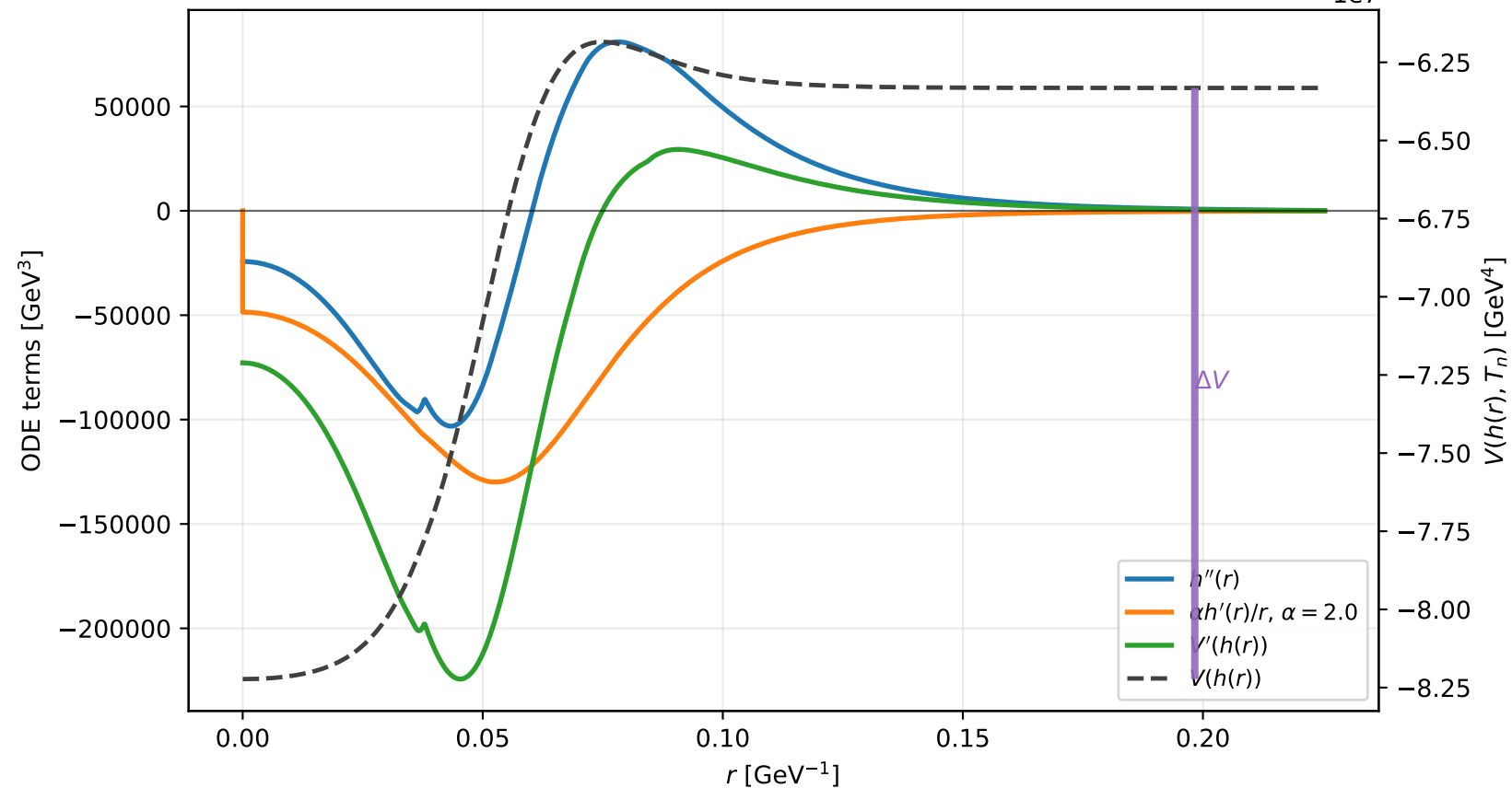
Example F7: bounce equation terms at T_n = 70.64 GeV
