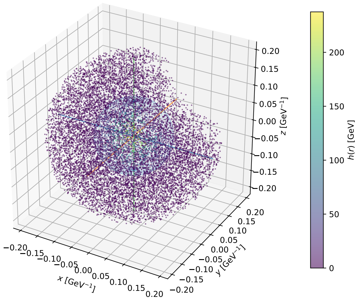
Example F5: 3D bubble profile at T_n = 63.98 GeV
