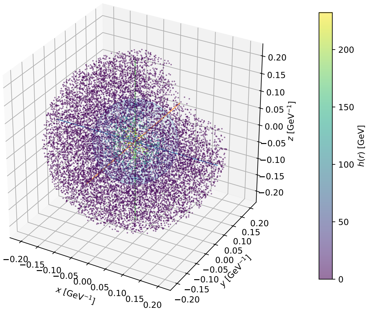
Example F5: 3D bubble profile at T_n = 72.88 GeV
