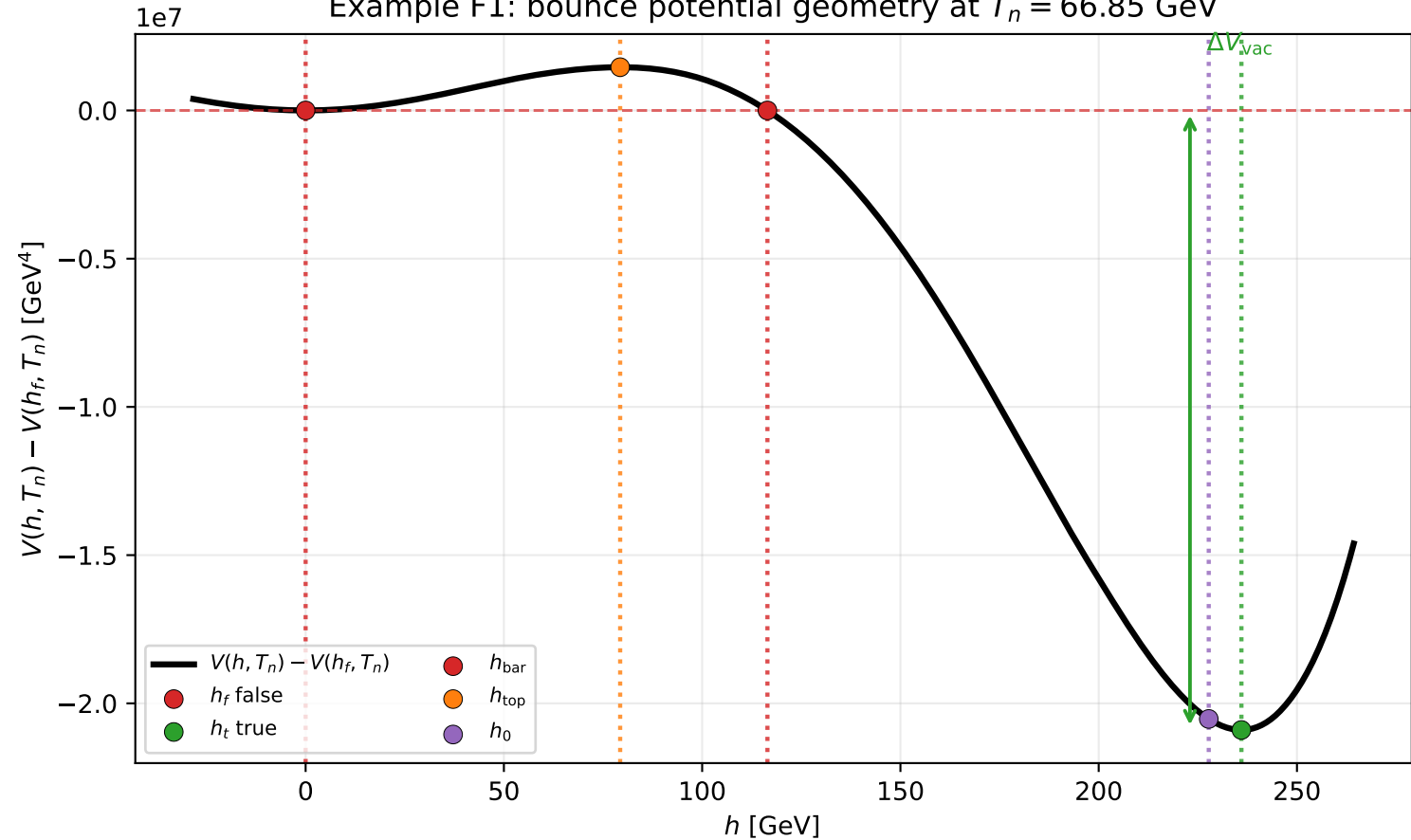
Example F1: bounce potential geometry at T_n = 66.85 GeV
