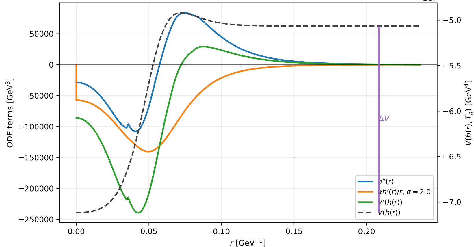
Example F7: bounce equation terms at T_n = 66.85 GeV
