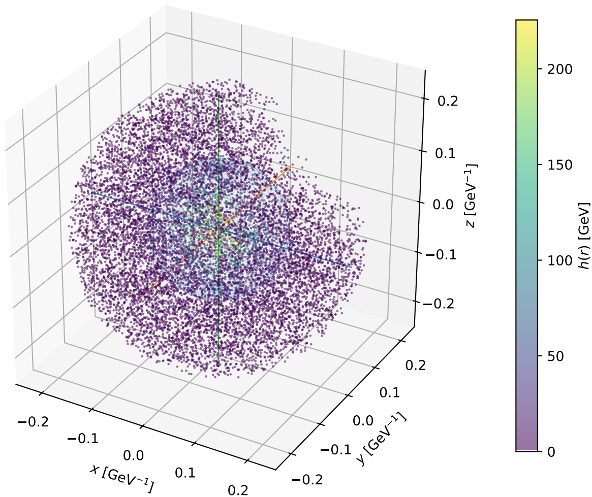
Example F5: 3D bubble profile at T_n = 80.59 GeV
