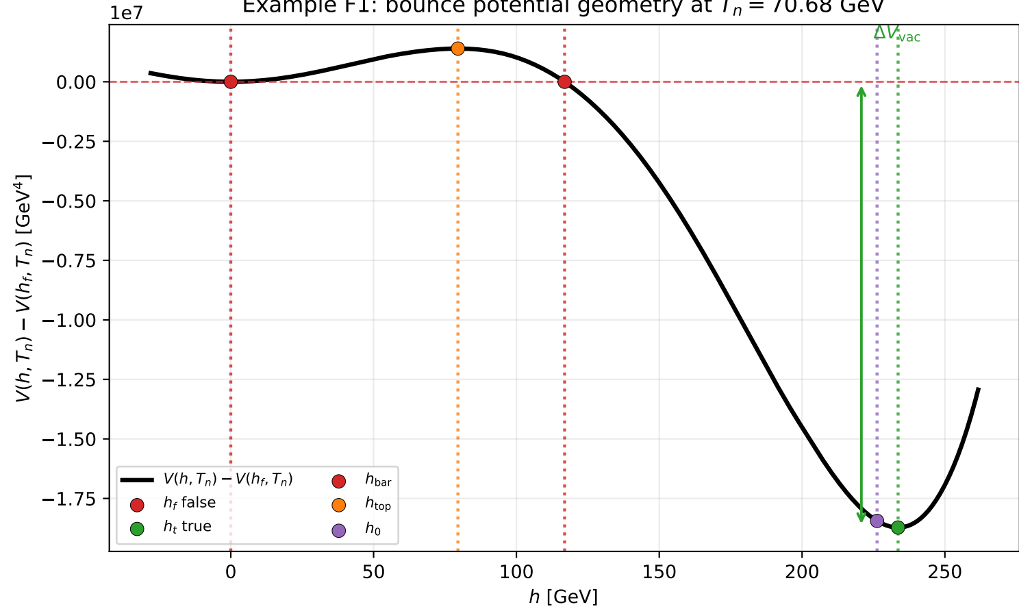
Example F1: bounce potential geometry at T_n = 70.68 GeV
