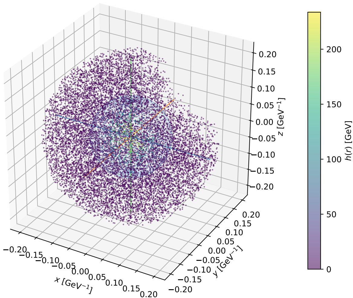
Example F5: 3D bubble profile at T_n = 70.68 GeV
