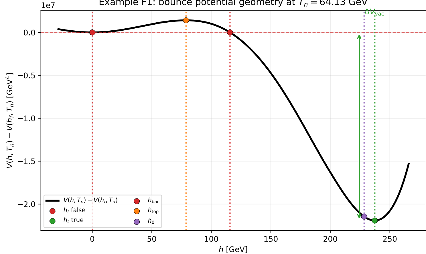
Example F1: bounce potential geometry at T_n = 64.13 GeV
