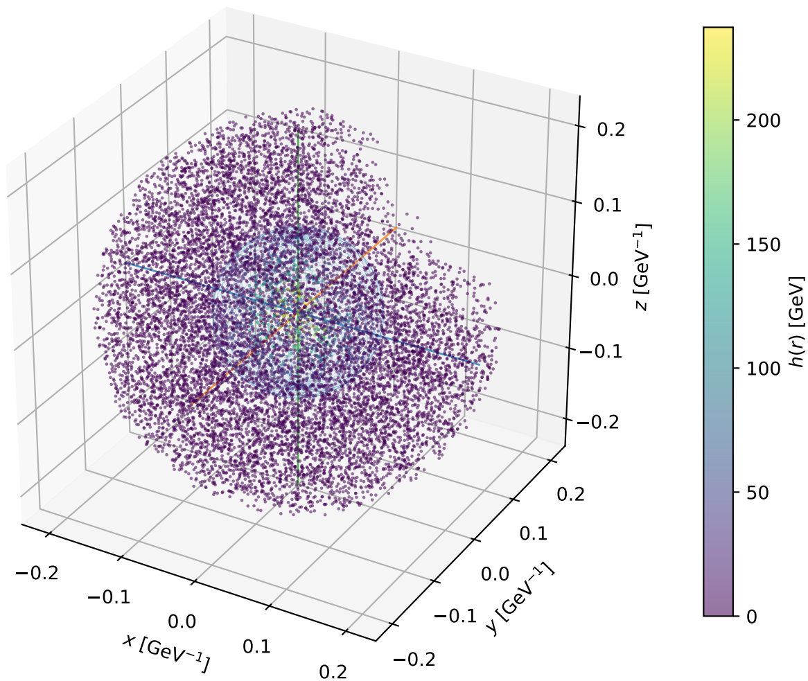
Example F5: 3D bubble profile at T_n = 64.13 GeV
