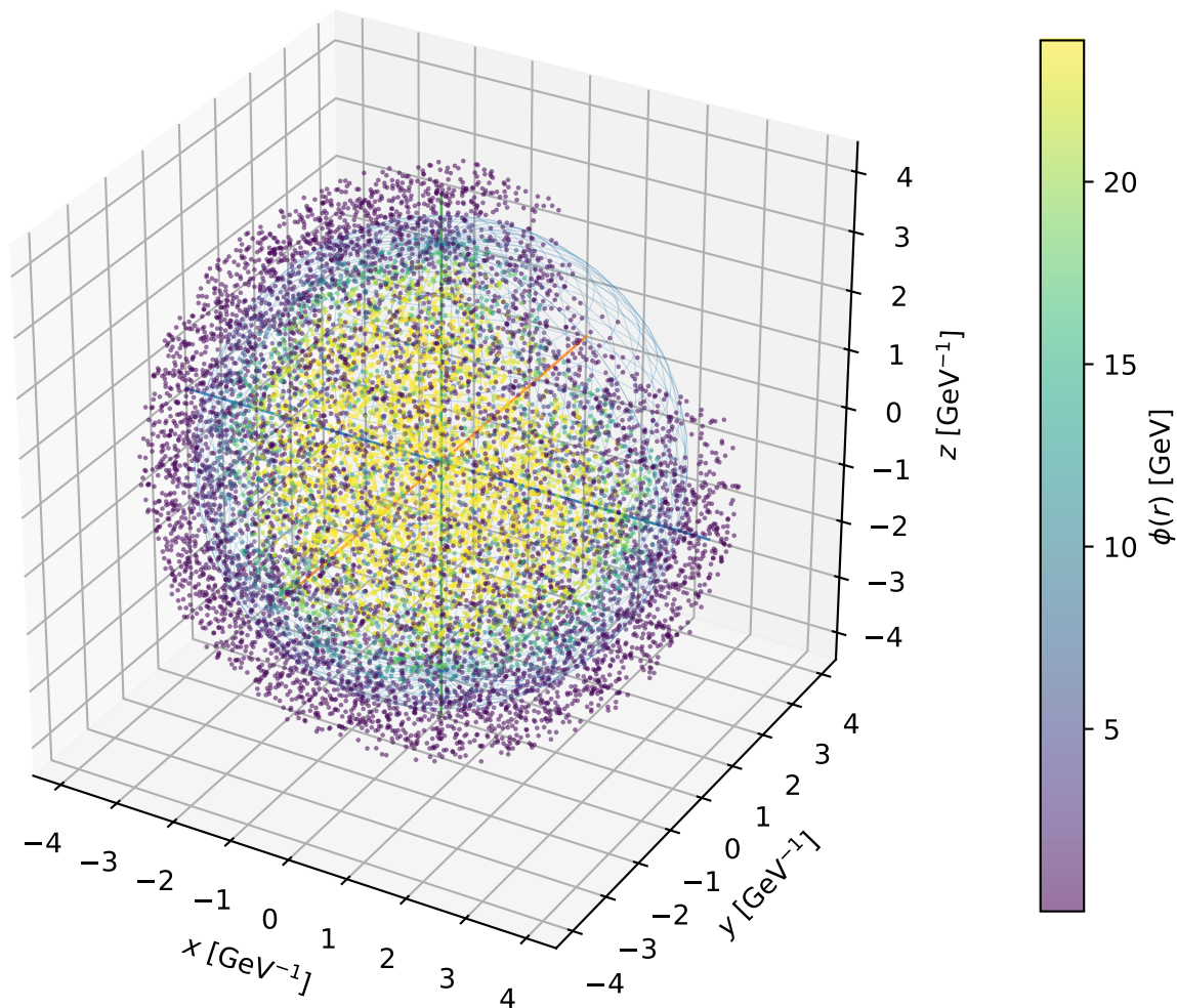
Example C5: 3D bubble profile at T_n = 166.9 GeV
